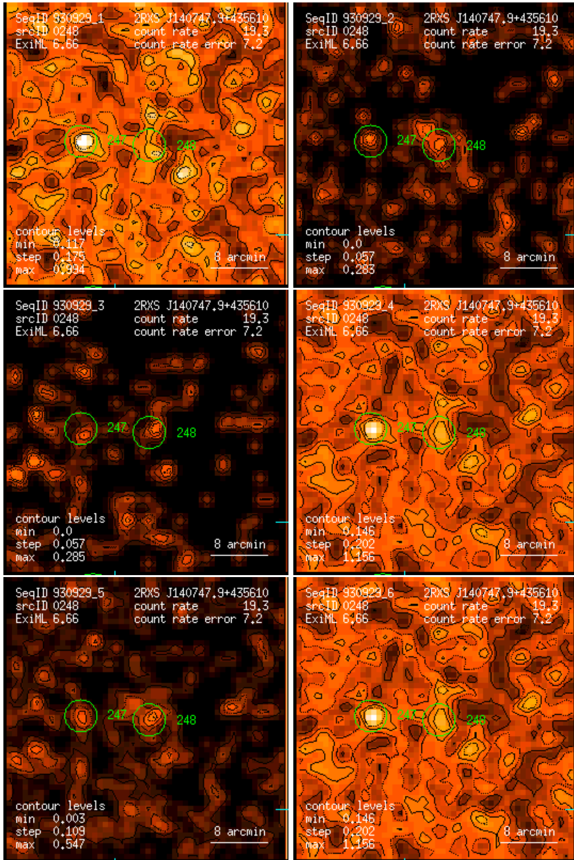
Figure 248: RASS 930929: detection 0248: band rate images, Gaussian filter: (1) PSPC channels 11 – 41, (2) 52 – 90, (3) 91 – 201, (4) 11 – 235, (5) 52 – 201, (6) 11 – 201. Broad band rates in counts/ks. Band rate contour levels in counts/ks/arcmin 2 .
