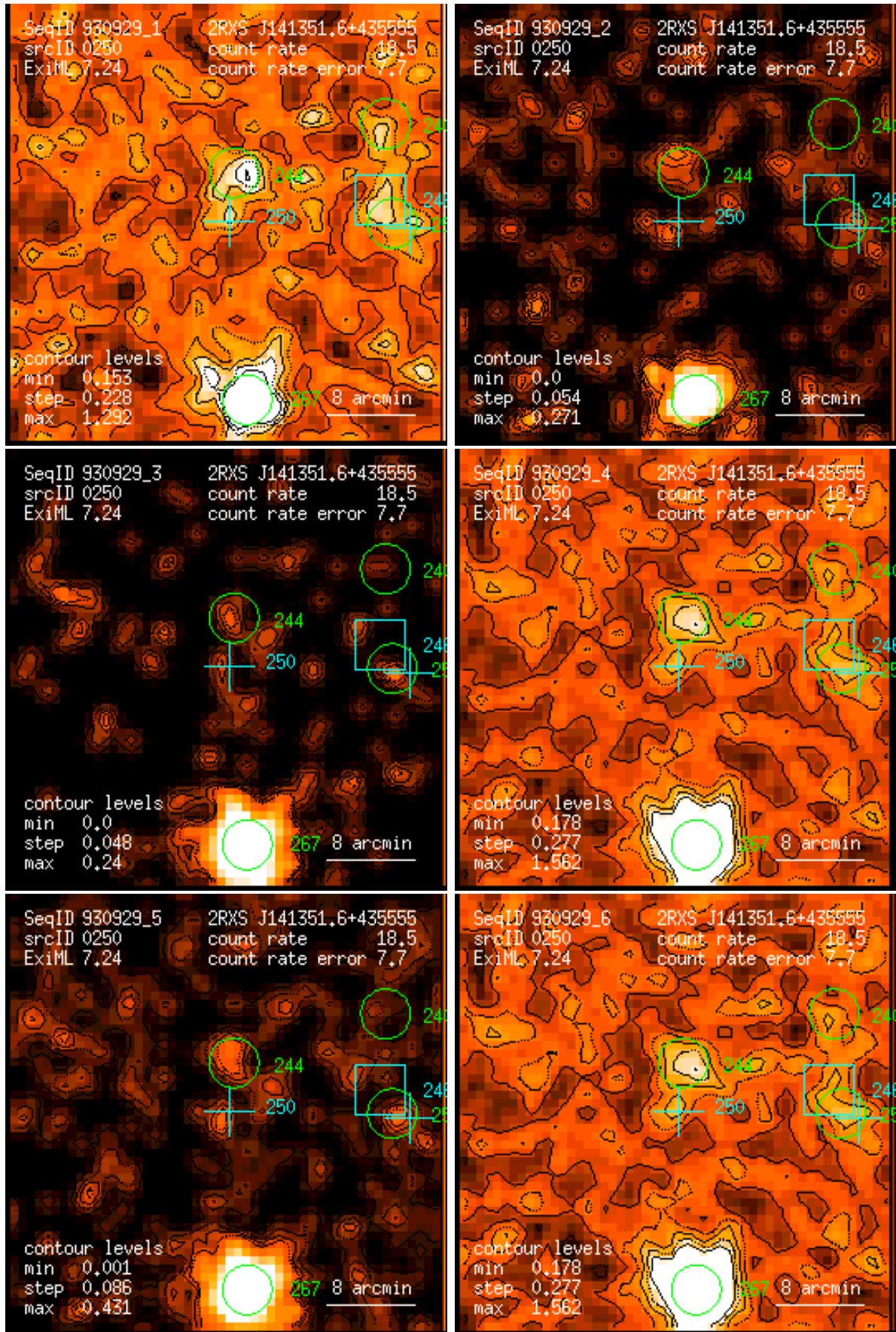
Figure 250: RASS 930929: detection 0250: band rate images, Gaussian filter: (1) PSPC channels 11 – 41, (2) 52 – 90, (3) 91 – 201, (4) 11 – 235, (5) 52 – 201, (6) 11 – 201. Broad band rates in counts/ks. Band rate contour levels in counts/ks/arcmin 2 .
