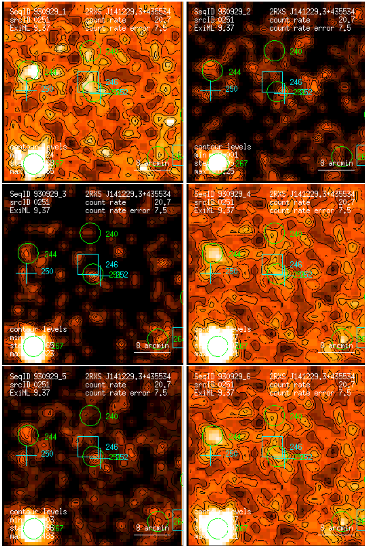
Figure 251: RASS 930929: detection 0251: band rate images, Gaussian filter: (1) PSPC channels 11 – 41, (2) 52 – 90, (3) 91 – 201, (4) 11 – 235, (5) 52 – 201, (6) 11 – 201. Broad band rates in counts/ks. Band rate contour levels in counts/ks/arcmin 2 .
