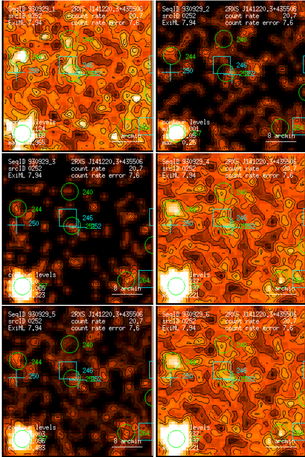
Figure 252: RASS 930929: detection 0252: band rate images, Gaussian filter: (1) PSPC channels 11 – 41, (2) 52 – 90, (3) 91 – 201, (4) 11 – 235, (5) 52 – 201, (6) 11 – 201. Broad band rates in counts/ks. Band rate contour levels in counts/ks/arcmin 2 .
