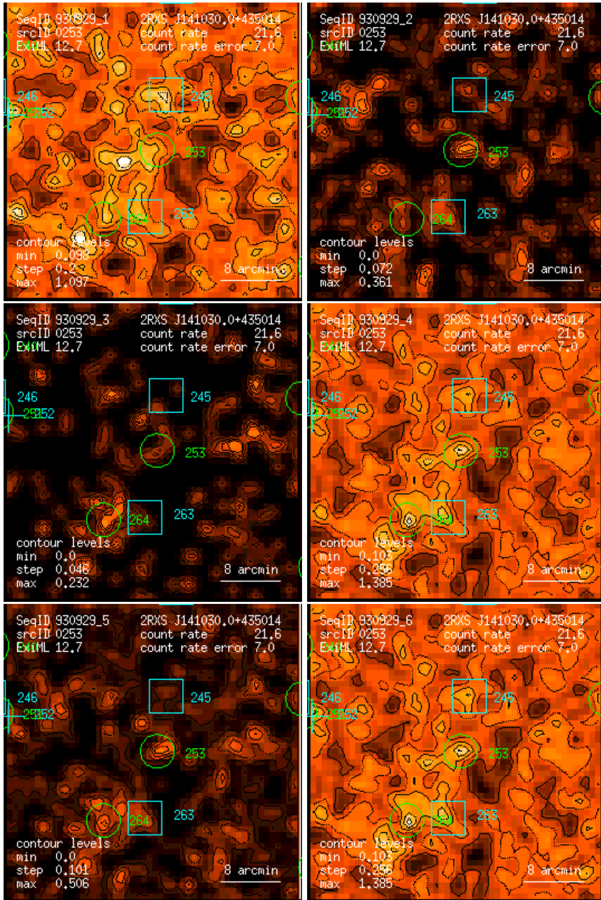
Figure 253: RASS 930929: detection 0253: band rate images, Gaussian filter: (1) PSPC channels 11 – 41, (2) 52 – 90, (3) 91 – 201, (4) 11 – 235, (5) 52 – 201, (6) 11 – 201. Broad band rates in counts/ks. Band rate contour levels in counts/ks/arcmin 2 .
