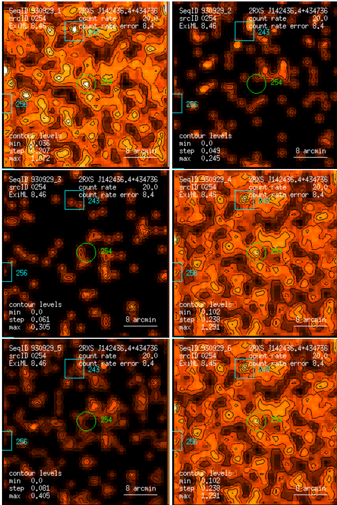
Figure 254: RASS 930929: detection 0254: band rate images, Gaussian filter: (1) PSPC channels 11 – 41, (2) 52 – 90, (3) 91 – 201, (4) 11 – 235, (5) 52 – 201, (6) 11 – 201. Broad band rates in counts/ks. Band rate contour levels in counts/ks/arcmin 2 .
