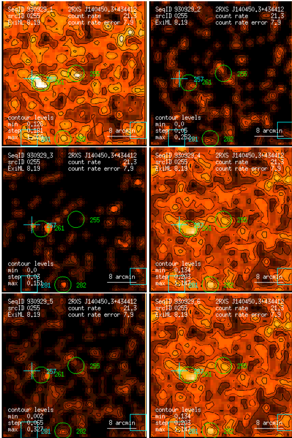
Figure 255: RASS 930929: detection 0255: band rate images, Gaussian filter: (1) PSPC channels 11 – 41, (2) 52 – 90, (3) 91 – 201, (4) 11 – 235, (5) 52 – 201, (6) 11 – 201. Broad band rates in counts/ks. Band rate contour levels in counts/ks/arcmin 2 .
