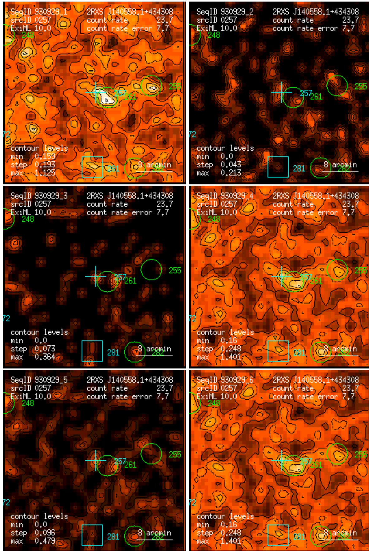
Figure 257: RASS 930929: detection 0257: band rate images, Gaussian filter: (1) PSPC channels 11 – 41, (2) 52 – 90, (3) 91 – 201, (4) 11 – 235, (5) 52 – 201, (6) 11 – 201. Broad band rates in counts/ks. Band rate contour levels in counts/ks/arcmin 2 .
