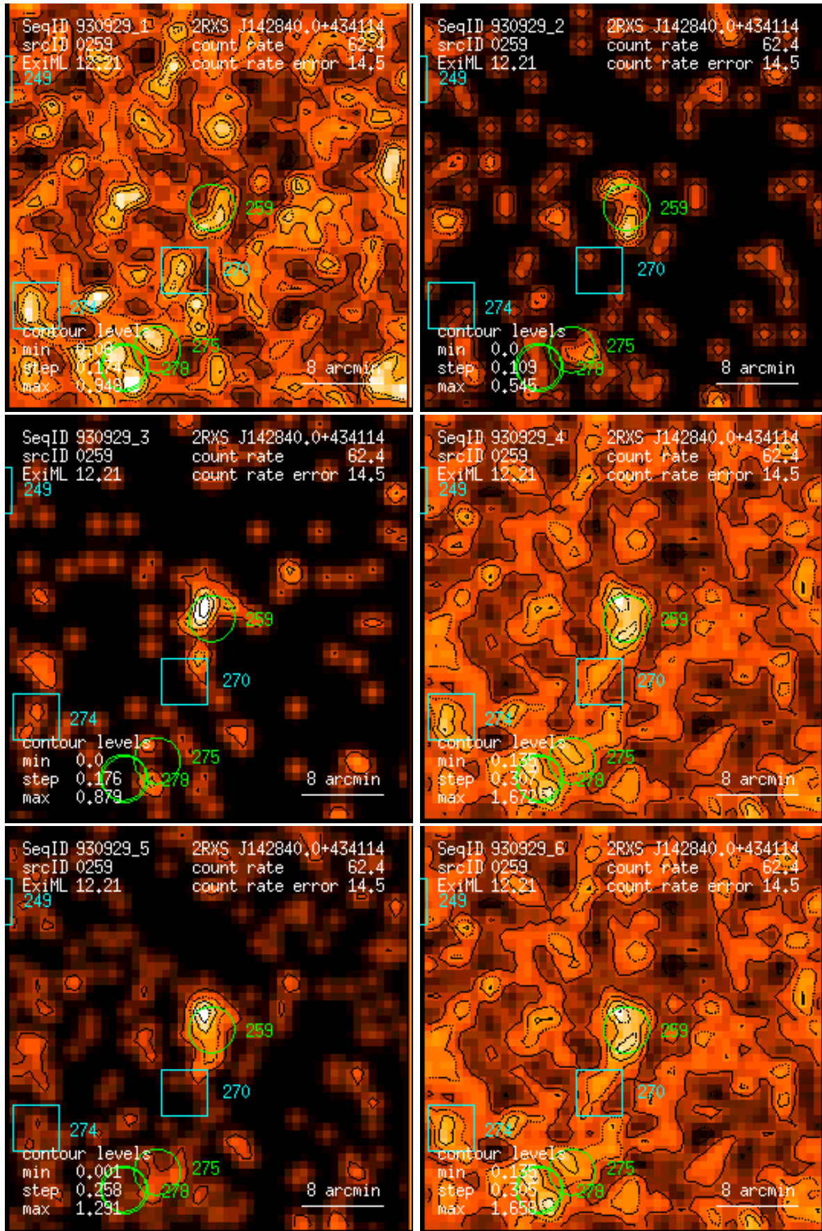
Figure 259: RASS 930929: detection 0259: band rate images, Gaussian filter: (1) PSPC channels 11 – 41, (2) 52 – 90, (3) 91 – 201, (4) 11 – 235, (5) 52 – 201, (6) 11 – 201. Broad band rates in counts/ks. Band rate contour levels in counts/ks/arcmin 2 .
