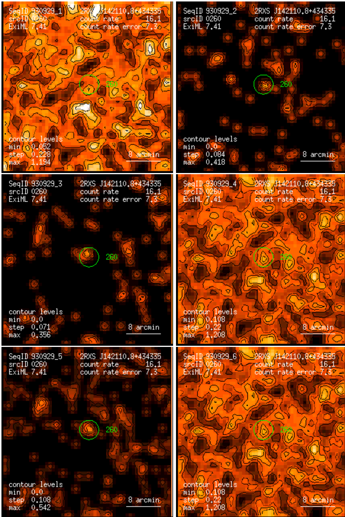
Figure 260: RASS 930929: detection 0260: band rate images, Gaussian filter: (1) PSPC channels 11 – 41, (2) 52 – 90, (3) 91 – 201, (4) 11 – 235, (5) 52 – 201, (6) 11 – 201. Broad band rates in counts/ks. Band rate contour levels in counts/ks/arcmin 2 .
