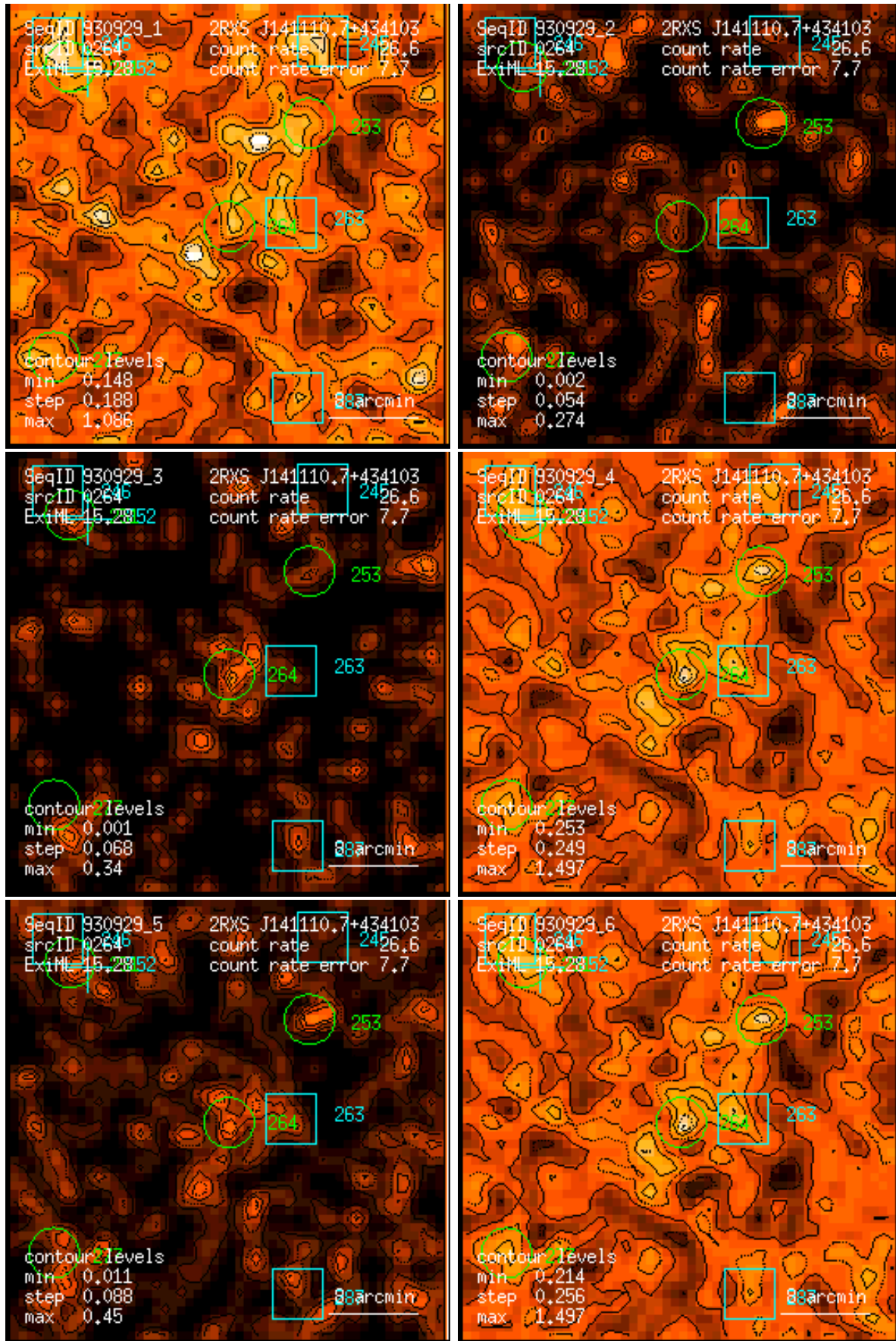
Figure 264: RASS 930929: detection 0264: band rate images, Gaussian filter: (1) PSPC channels 11 – 41, (2) 52 – 90, (3) 91 – 201, (4) 11 – 235, (5) 52 – 201, (6) 11 – 201. Broad band rates in counts/ks. Band rate contour levels in counts/ks/arcmin 2 .
