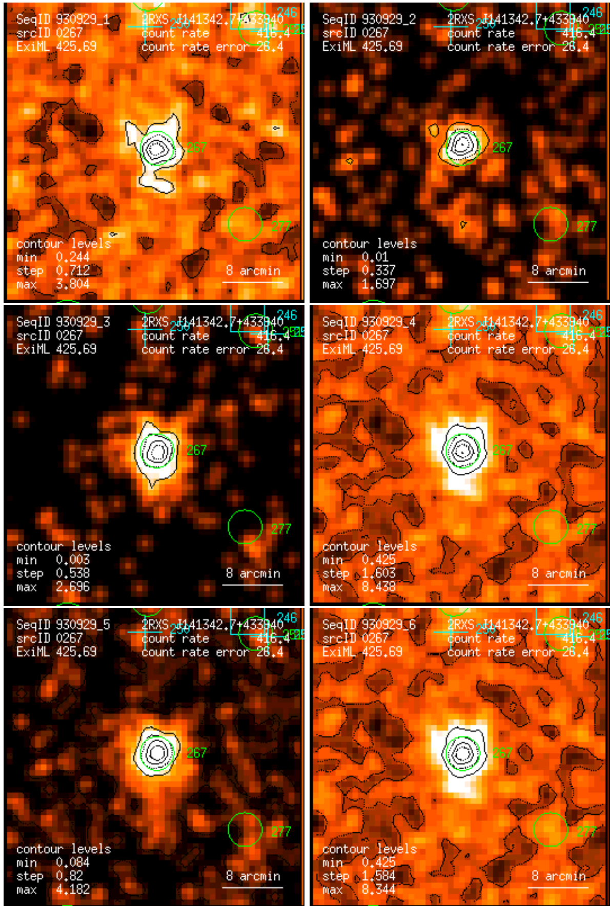
Figure 267: RASS 930929: detection 0267: band rate images, Gaussian filter: (1) PSPC channels 11 – 41, (2) 52 – 90, (3) 91 – 201, (4) 11 – 235, (5) 52 – 201, (6) 11 – 201. Broad band rates in counts/ks. Band rate contour levels in counts/ks/arcmin 2 .
