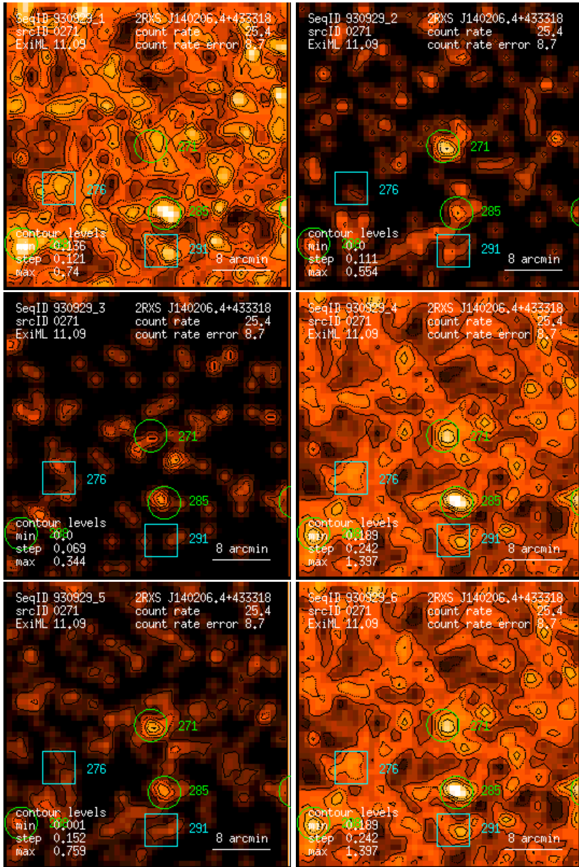
Figure 271: RASS 930929: detection 0271: band rate images, Gaussian filter: (1) PSPC channels 11 – 41, (2) 52 – 90, (3) 91 – 201, (4) 11 – 235, (5) 52 – 201, (6) 11 – 201. Broad band rates in counts/ks. Band rate contour levels in counts/ks/arcmin 2 .
