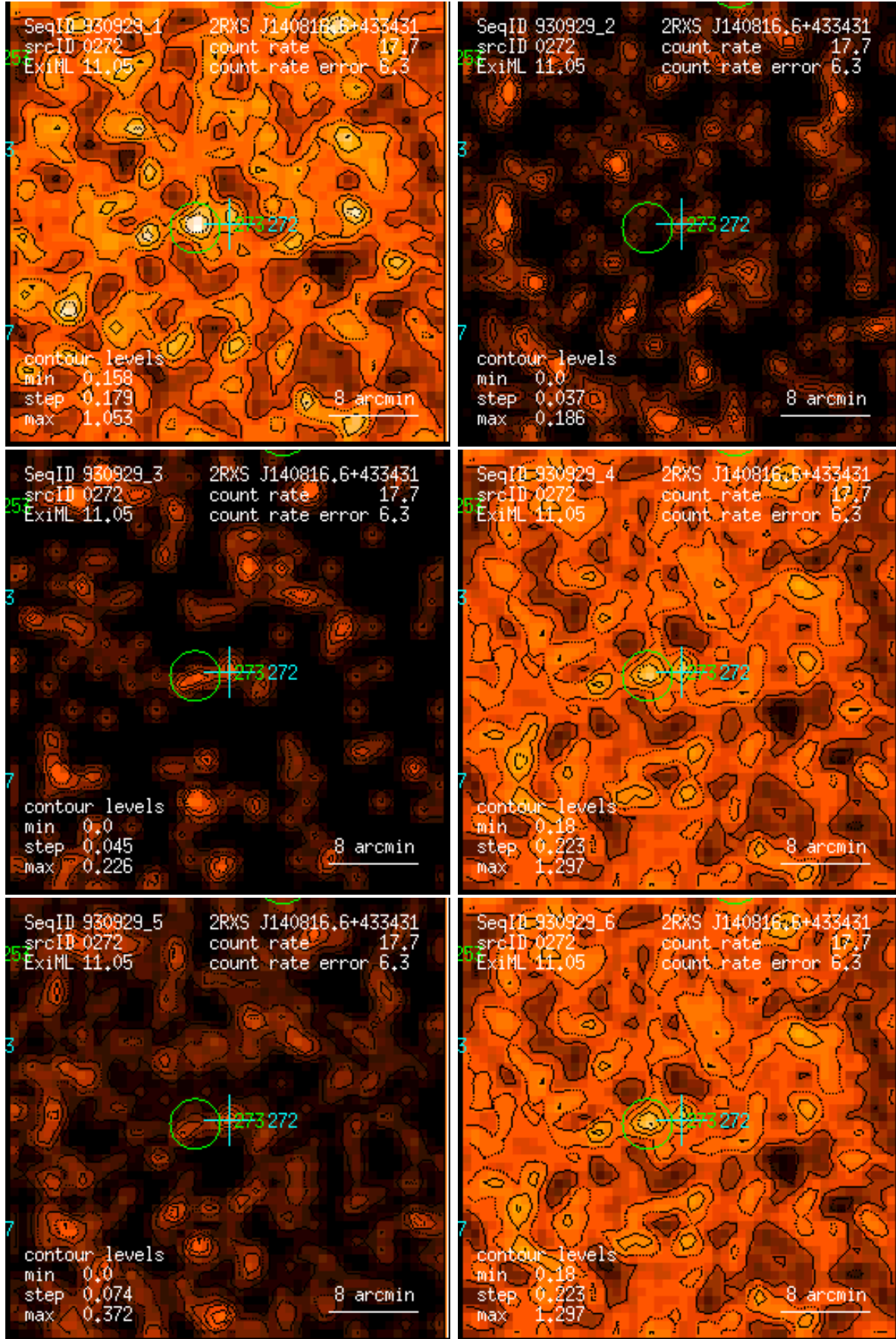
Figure 272: RASS 930929: detection 0272: band rate images, Gaussian filter: (1) PSPC channels 11 – 41, (2) 52 – 90, (3) 91 – 201, (4) 11 – 235, (5) 52 – 201, (6) 11 – 201. Broad band rates in counts/ks. Band rate contour levels in counts/ks/arcmin 2 .
