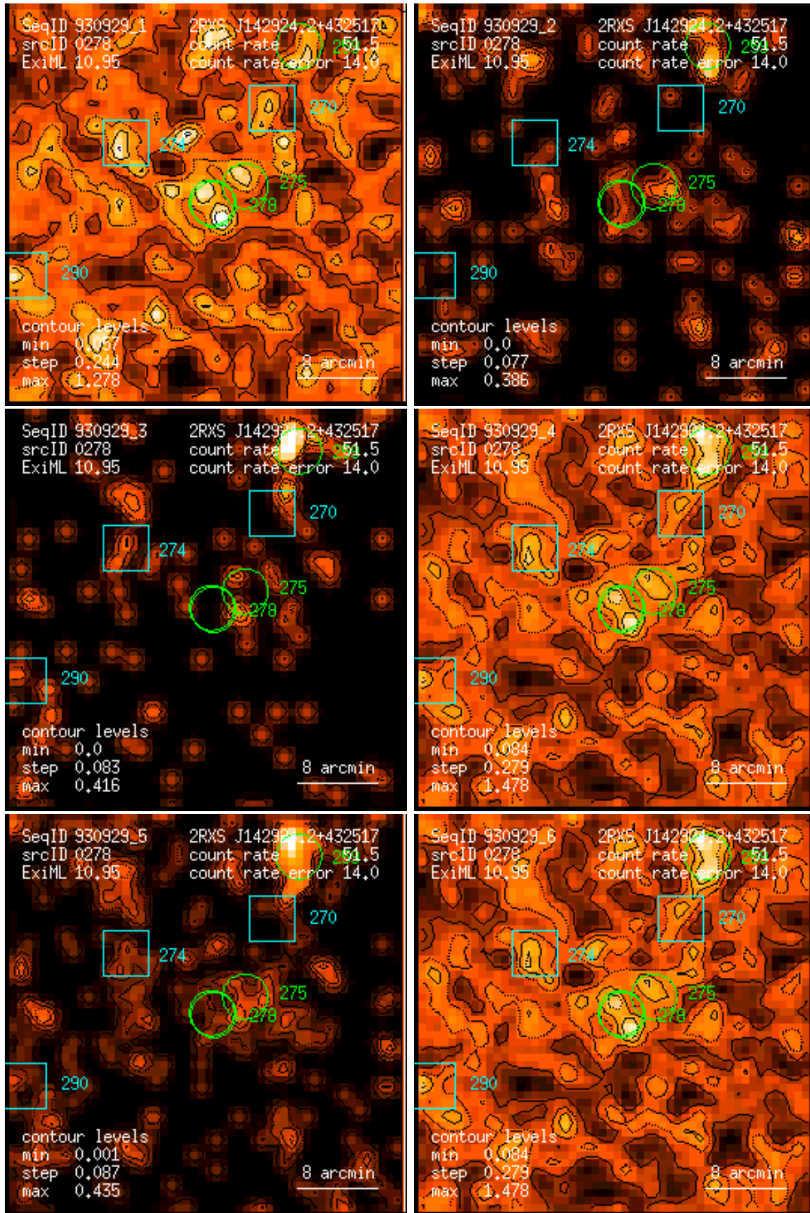
Figure 278: RASS 930929: detection 0278: band rate images, Gaussian filter: (1) PSPC channels 11 – 41, (2) 52 – 90, (3) 91 – 201, (4) 11 – 235, (5) 52 – 201, (6) 11 – 201. Broad band rates in counts/ks. Band rate contour levels in counts/ks/arcmin 2 .
