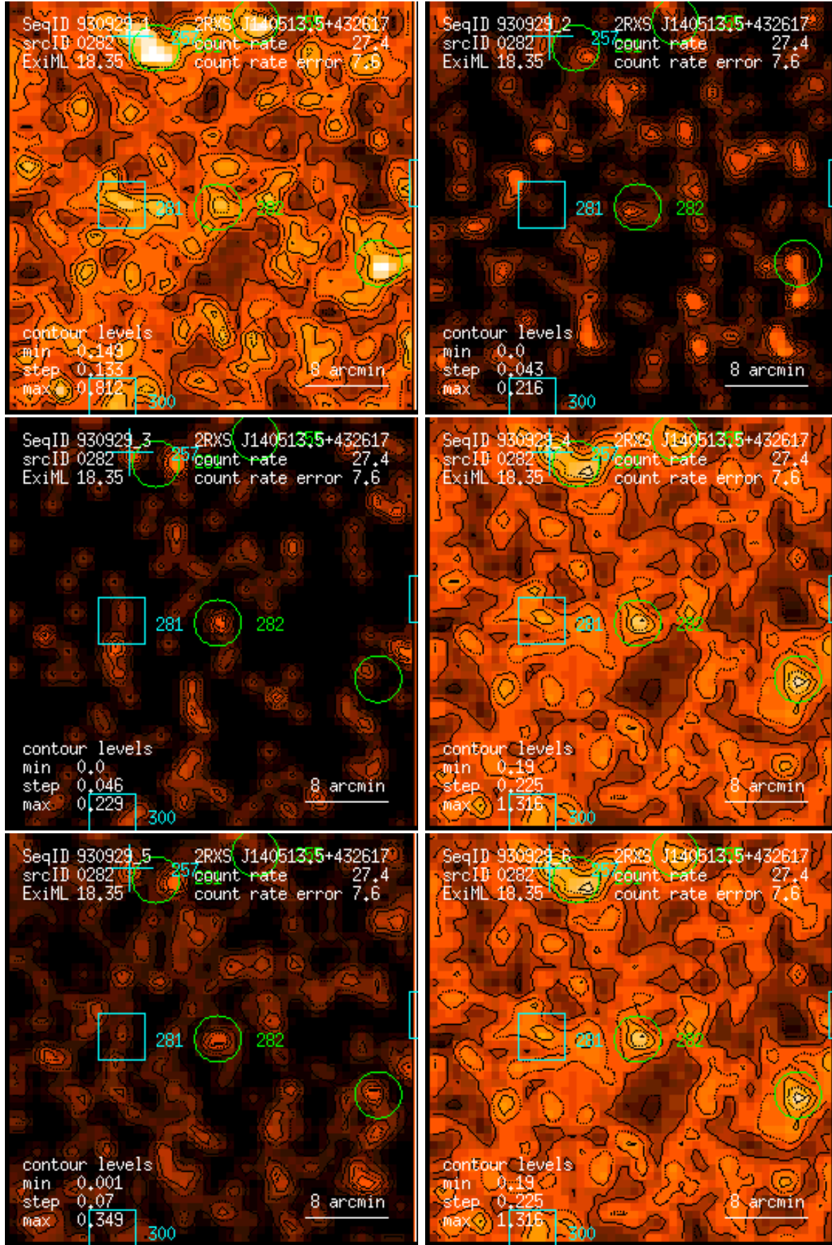
Figure 282: RASS 930929: detection 0282: band rate images, Gaussian filter: (1) PSPC channels 11 – 41, (2) 52 – 90, (3) 91 – 201, (4) 11 – 235, (5) 52 – 201, (6) 11 – 201. Broad band rates in counts/ks. Band rate contour levels in counts/ks/arcmin 2 .
