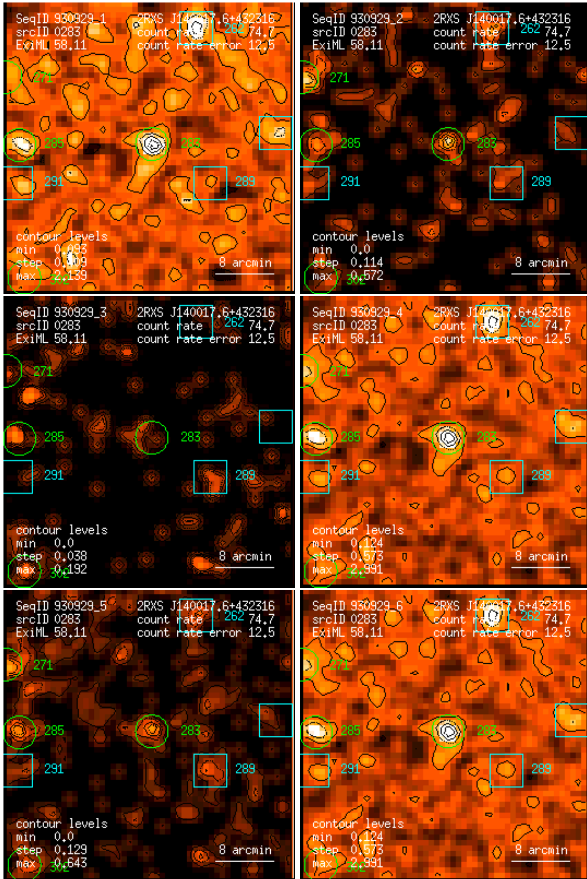
Figure 283: RASS 930929: detection 0283: band rate images, Gaussian filter: (1) PSPC channels 11 – 41, (2) 52 – 90, (3) 91 – 201, (4) 11 – 235, (5) 52 – 201, (6) 11 – 201. Broad band rates in counts/ks. Band rate contour levels in counts/ks/arcmin 2 .
