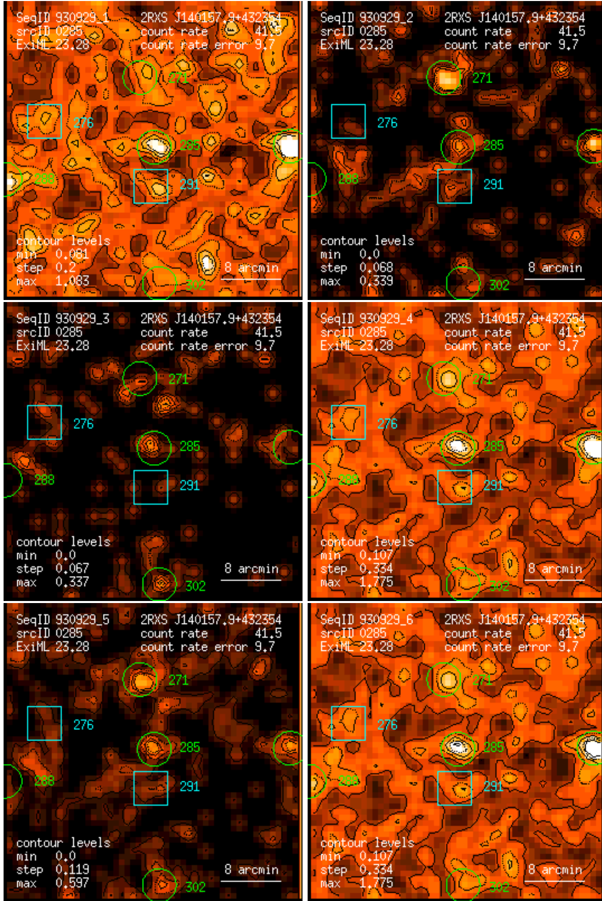
Figure 285: RASS 930929: detection 0285: band rate images, Gaussian filter: (1) PSPC channels 11 – 41, (2) 52 – 90, (3) 91 – 201, (4) 11 – 235, (5) 52 – 201, (6) 11 – 201. Broad band rates in counts/ks. Band rate contour levels in counts/ks/arcmin 2 .
