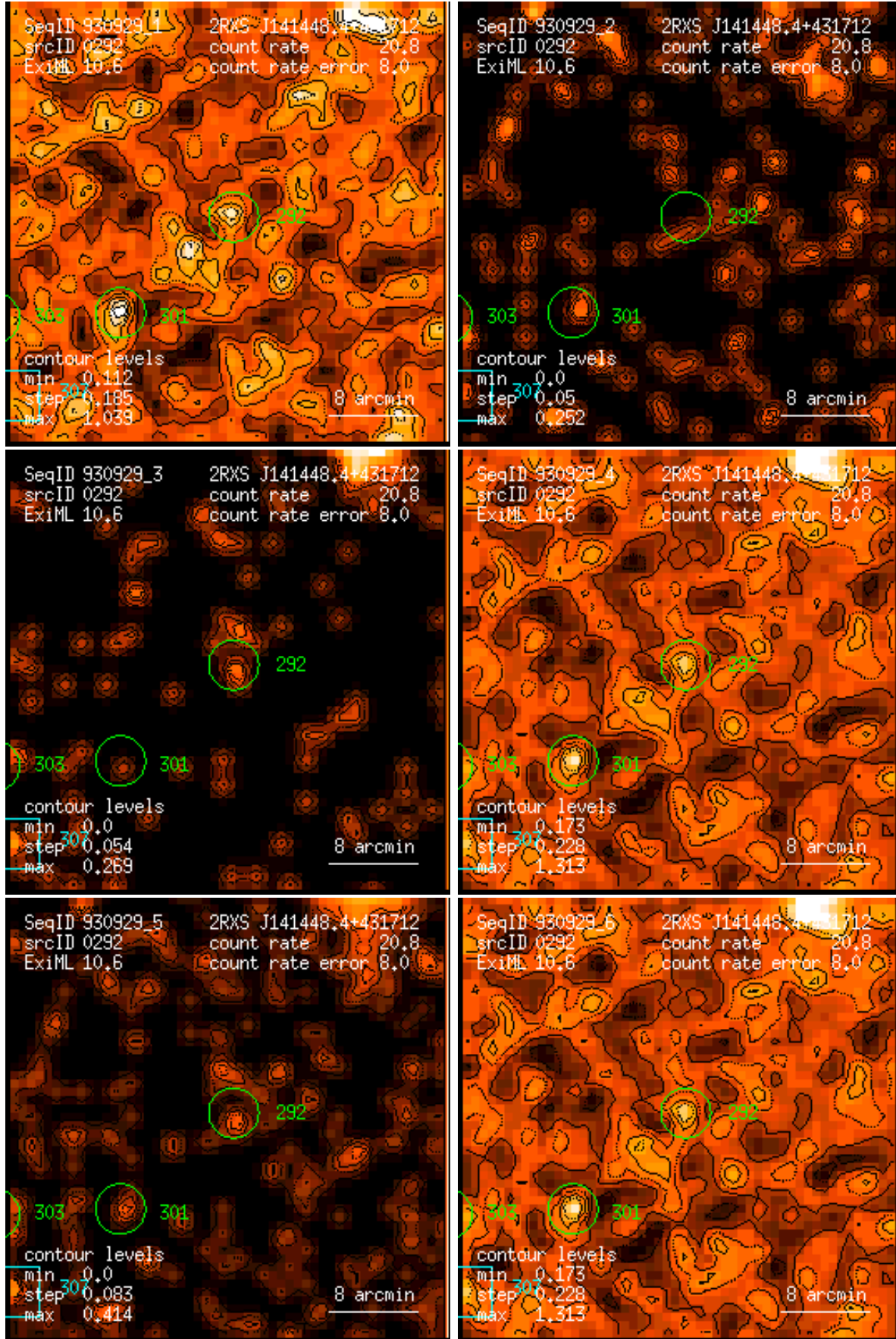
Figure 292: RASS 930929: detection 0292: band rate images, Gaussian filter: (1) PSPC channels 11 – 41, (2) 52 – 90, (3) 91 – 201, (4) 11 – 235, (5) 52 – 201, (6) 11 – 201. Broad band rates in counts/ks. Band rate contour levels in counts/ks/arcmin 2 .
