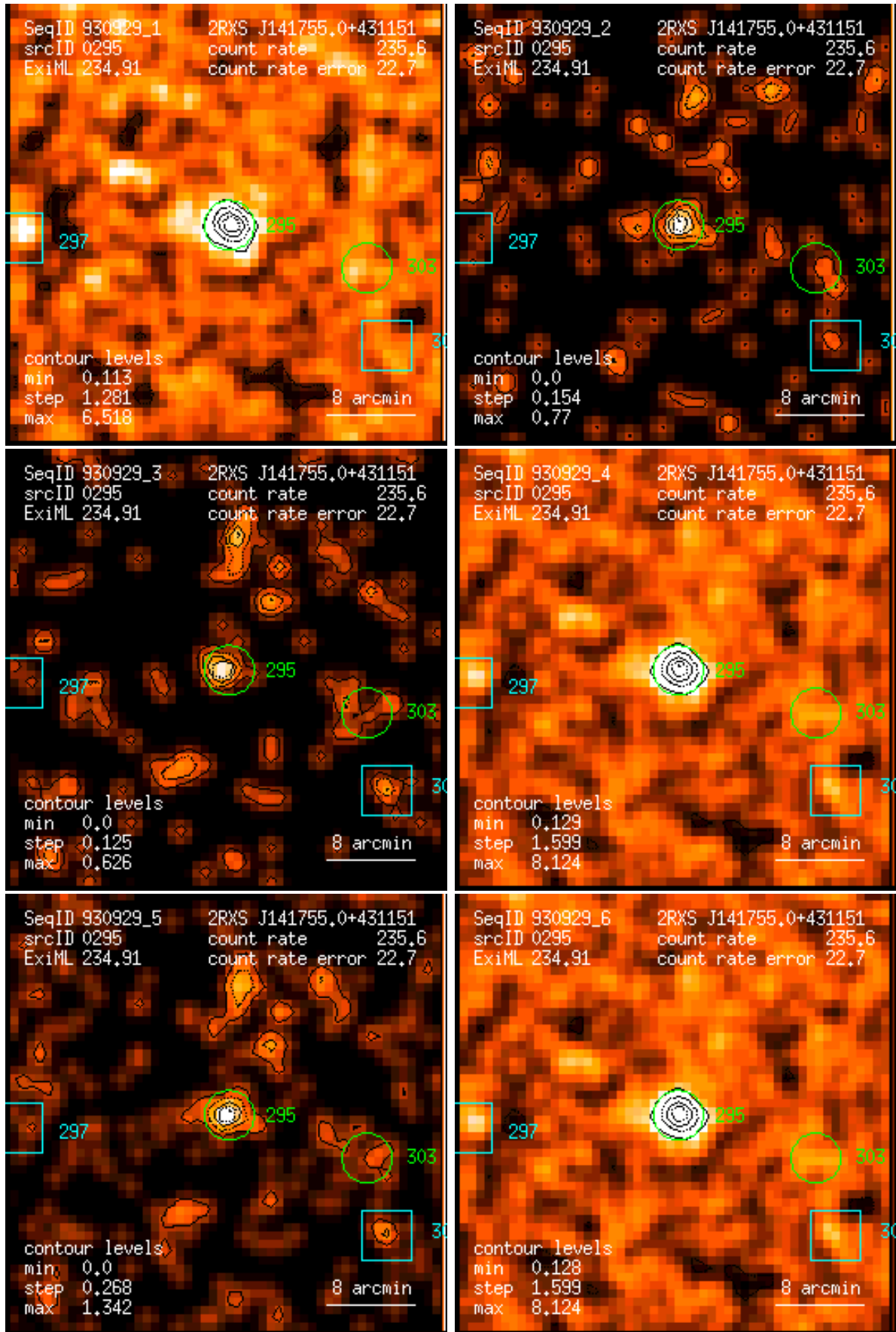
Figure 295: RASS 930929: detection 0295: band rate images, Gaussian filter: (1) PSPC channels 11 – 41, (2) 52 – 90, (3) 91 – 201, (4) 11 – 235, (5) 52 – 201, (6) 11 – 201. Broad band rates in counts/ks. Band rate contour levels in counts/ks/arcmin 2 .
