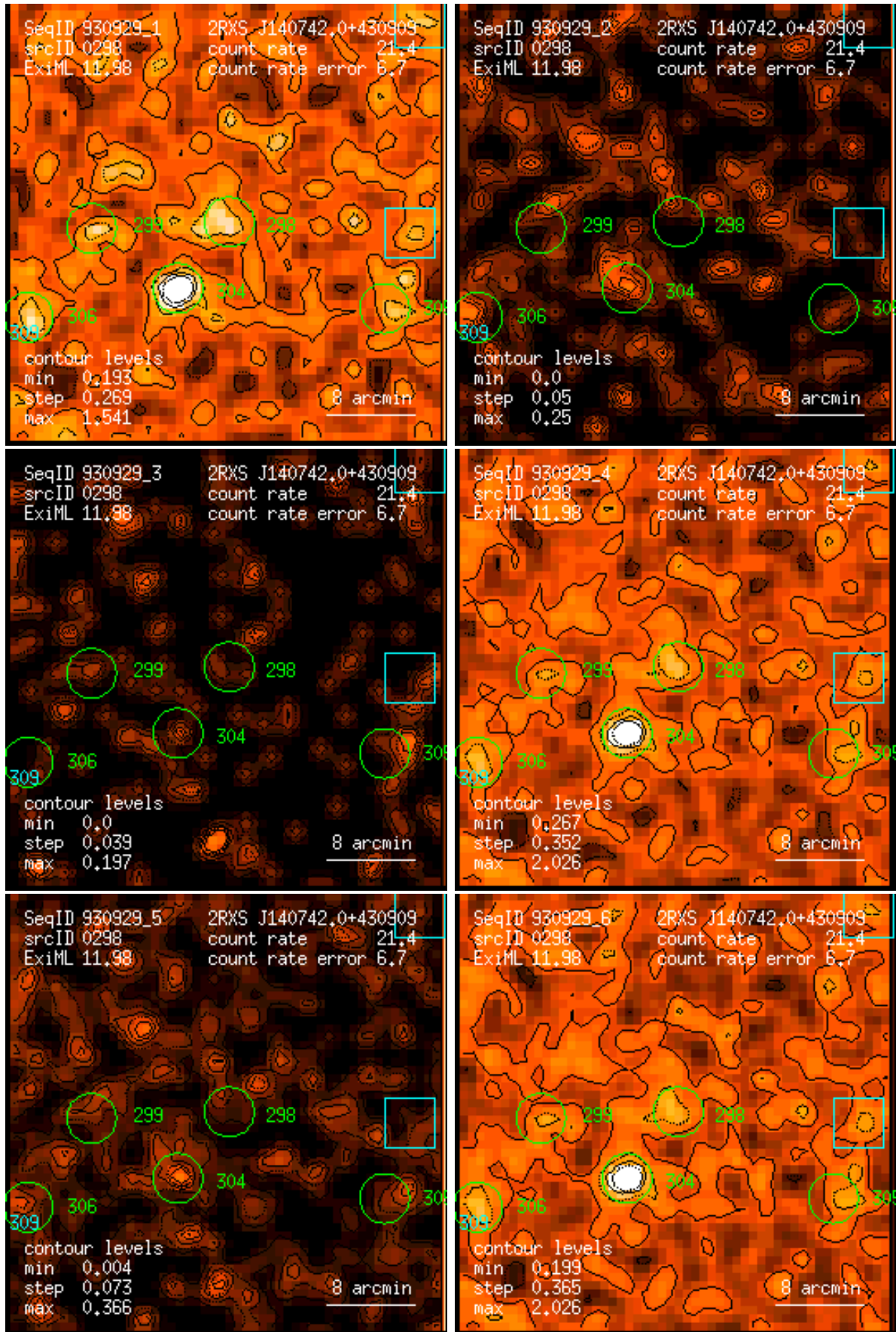
Figure 298: RASS 930929: detection 0298: band rate images, Gaussian filter: (1) PSPC channels 11 – 41, (2) 52 – 90, (3) 91 – 201, (4) 11 – 235, (5) 52 – 201, (6) 11 – 201. Broad band rates in counts/ks. Band rate contour levels in counts/ks/arcmin 2 .
