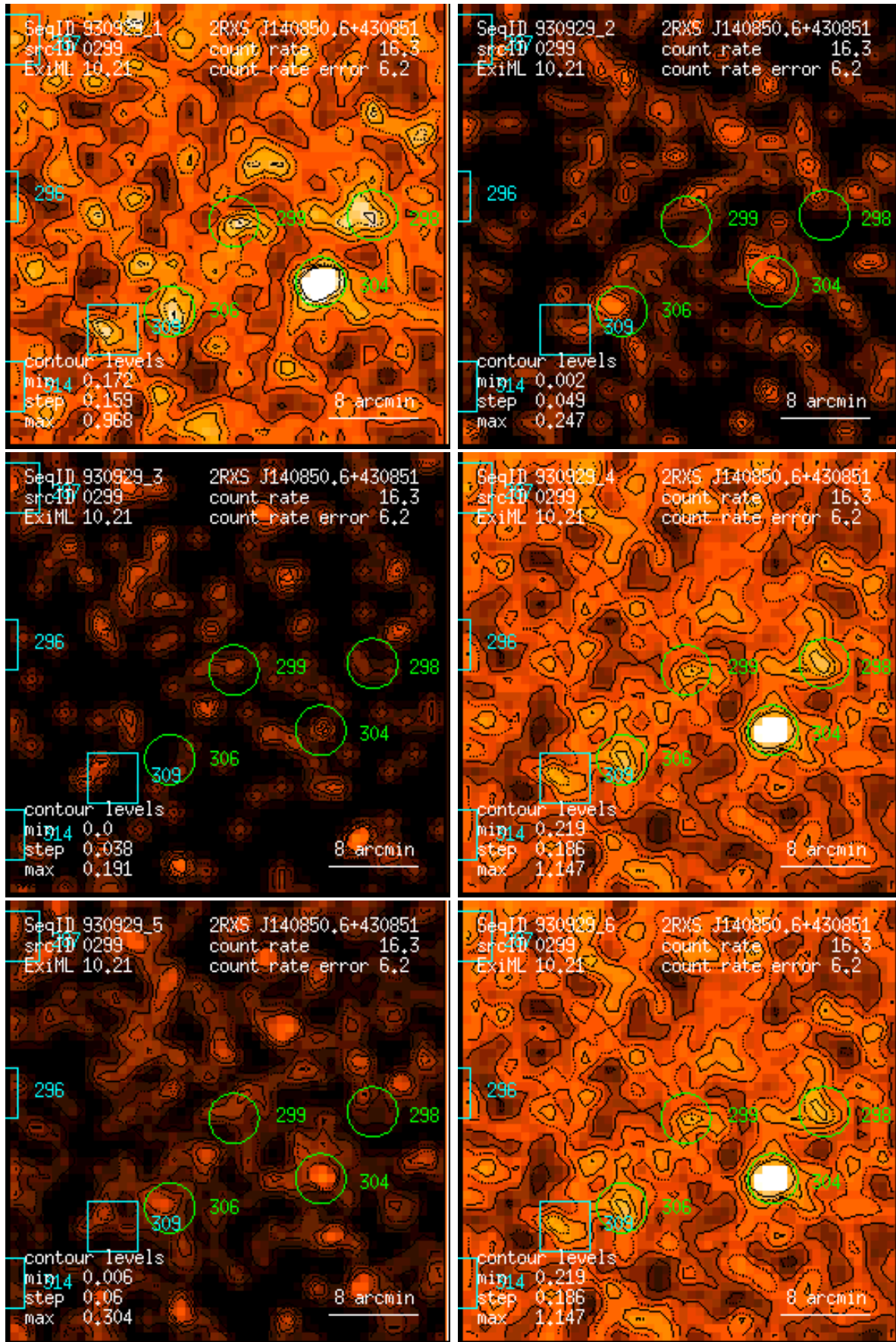
Figure 299: RASS 930929: detection 0299: band rate images, Gaussian filter: (1) PSPC channels 11 – 41, (2) 52 – 90, (3) 91 – 201, (4) 11 – 235, (5) 52 – 201, (6) 11 – 201. Broad band rates in counts/ks. Band rate contour levels in counts/ks/arcmin 2 .
