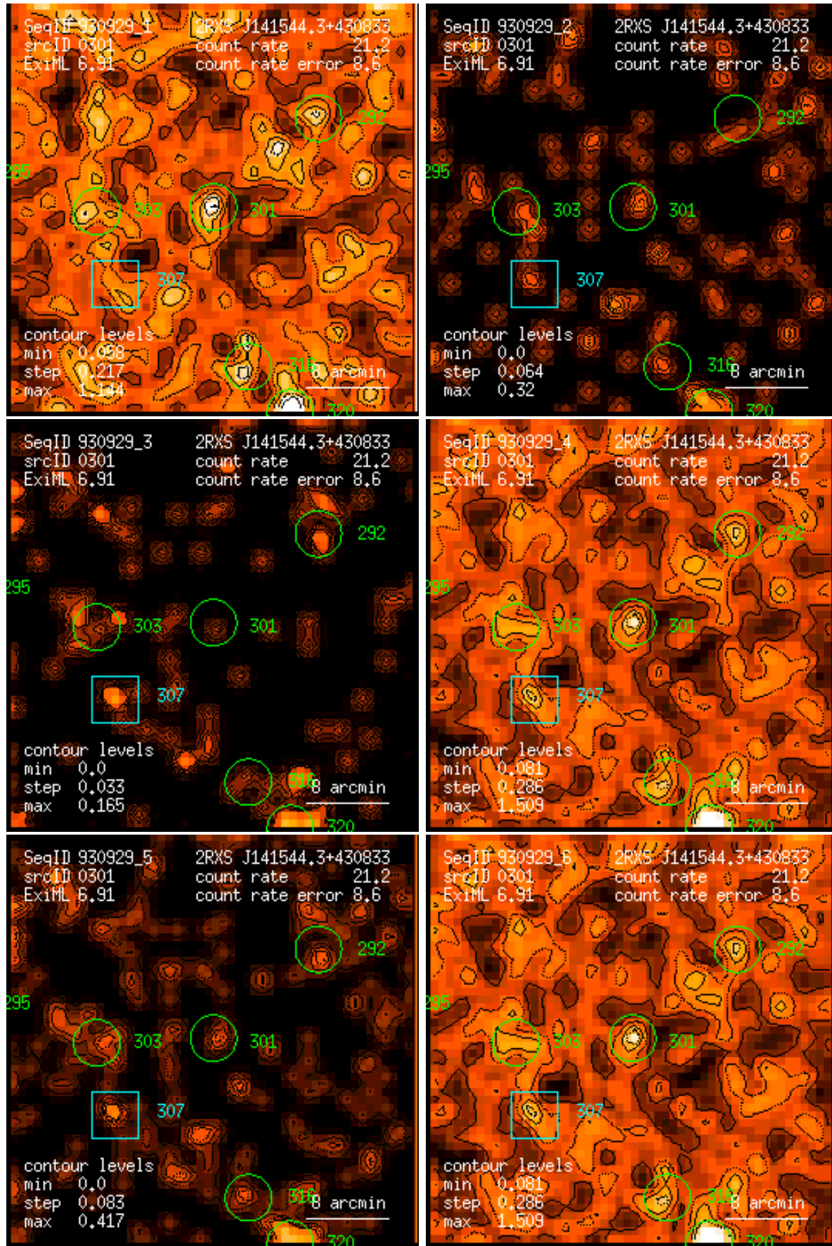
Figure 301: RASS 930929: detection 0301: band rate images, Gaussian filter: (1) PSPC channels 11 – 41, (2) 52 – 90, (3) 91 – 201, (4) 11 – 235, (5) 52 – 201, (6) 11 – 201. Broad band rates in counts/ks. Band rate contour levels in counts/ks/arcmin 2 .
