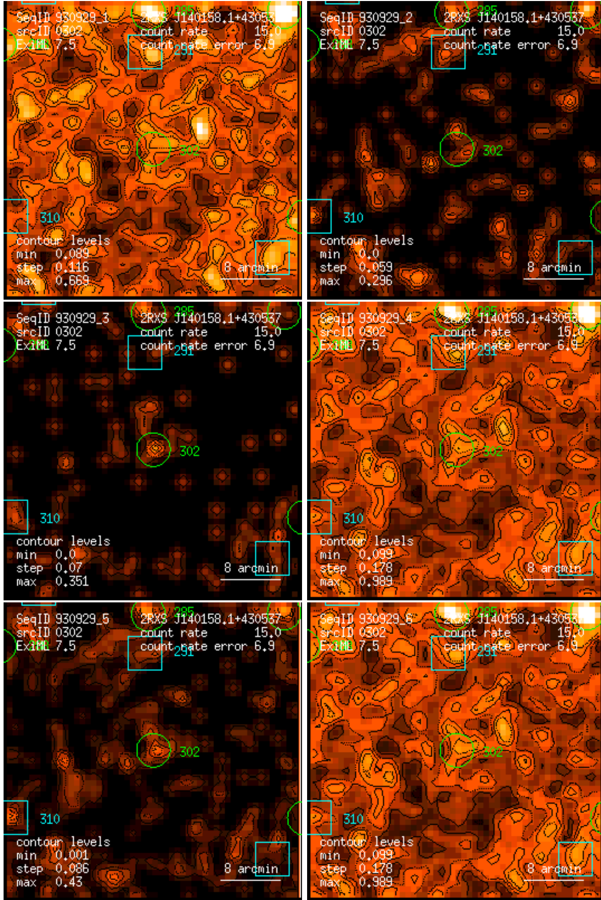
Figure 302: RASS 930929: detection 0302: band rate images, Gaussian filter: (1) PSPC channels 11 – 41, (2) 52 – 90, (3) 91 – 201, (4) 11 – 235, (5) 52 – 201, (6) 11 – 201. Broad band rates in counts/ks. Band rate contour levels in counts/ks/arcmin 2 .
