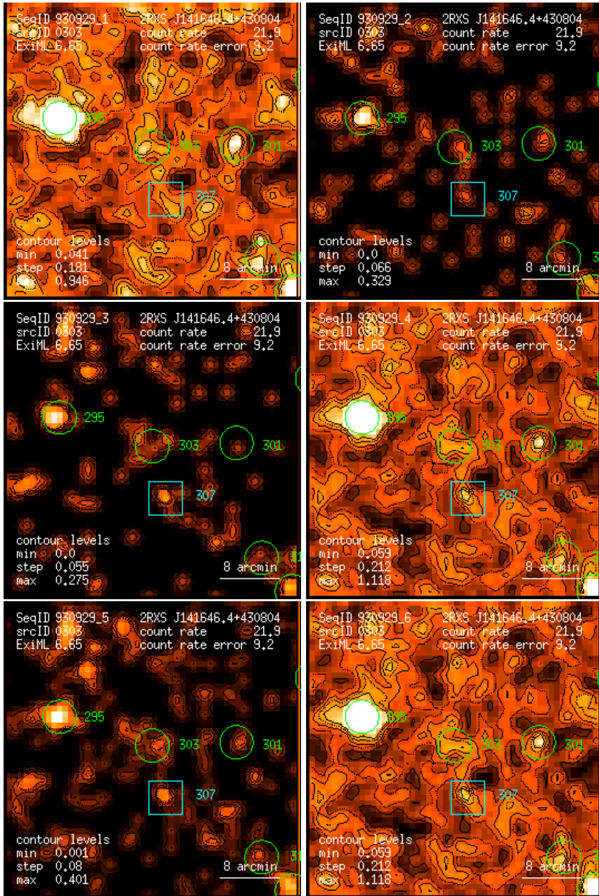
Figure 303: RASS 930929: detection 0303: band rate images, Gaussian filter: (1) PSPC channels 11 – 41, (2) 52 – 90, (3) 91 – 201, (4) 11 – 235, (5) 52 – 201, (6) 11 – 201. Broad band rates in counts/ks. Band rate contour levels in counts/ks/arcmin 2 .
