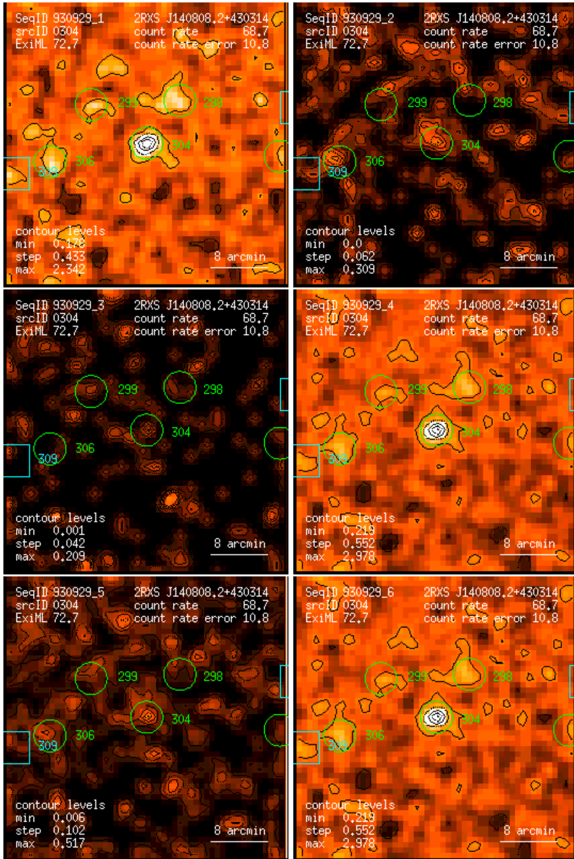
Figure 304: RASS 930929: detection 0304: band rate images, Gaussian filter: (1) PSPC channels 11 – 41, (2) 52 – 90, (3) 91 – 201, (4) 11 – 235, (5) 52 – 201, (6) 11 – 201. Broad band rates in counts/ks. Band rate contour levels in counts/ks/arcmin 2 .
