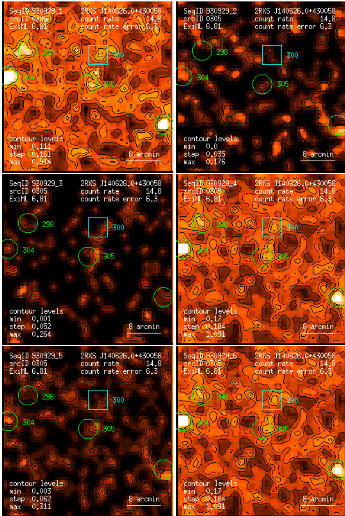
Figure 305: RASS 930929: detection 0305: band rate images, Gaussian filter: (1) PSPC channels 11 – 41, (2) 52 – 90, (3) 91 – 201, (4) 11 – 235, (5) 52 – 201, (6) 11 – 201. Broad band rates in counts/ks. Band rate contour levels in counts/ks/arcmin 2 .
