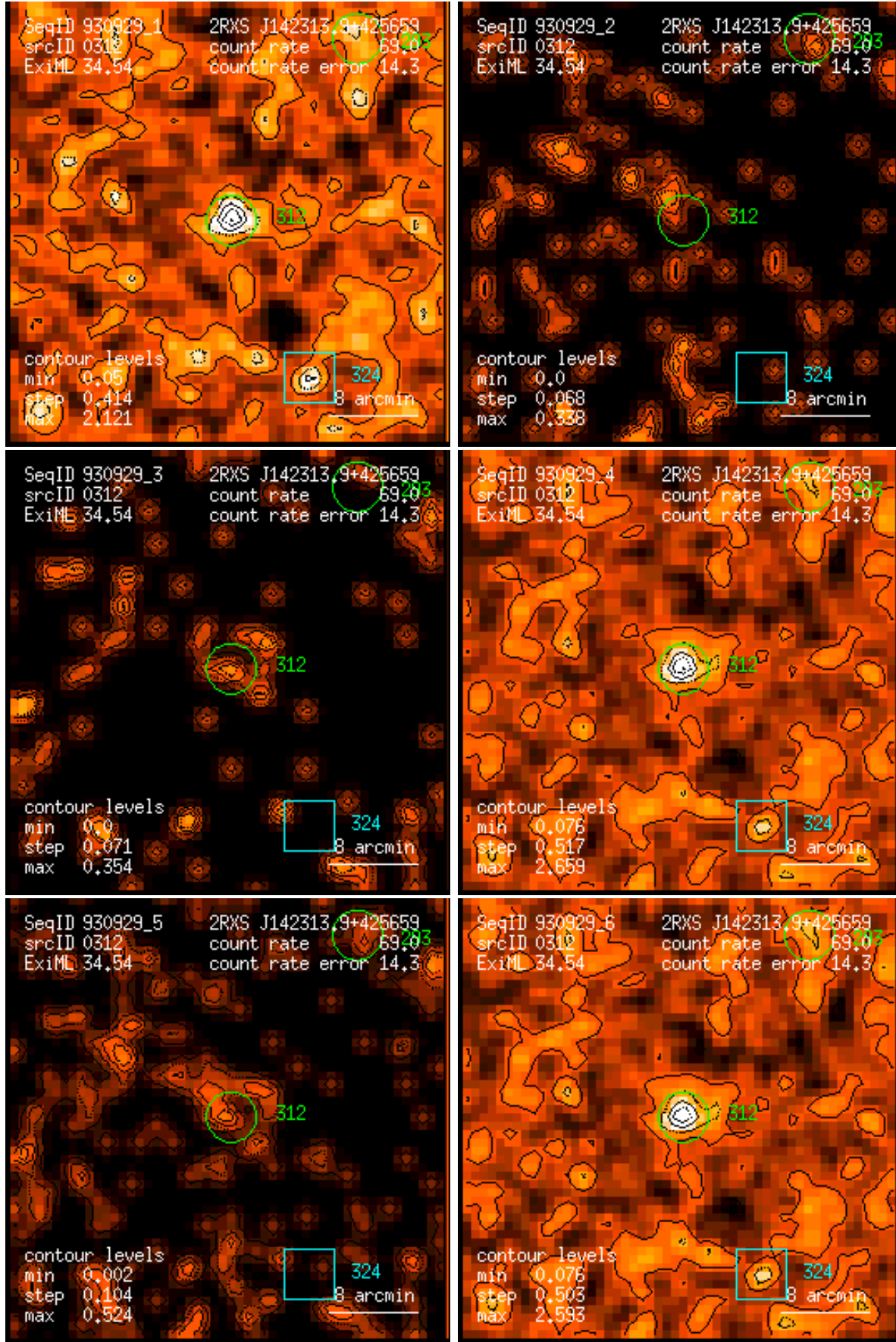
Figure 312: RASS 930929: detection 0312: band rate images, Gaussian filter: (1) PSPC channels 11 – 41, (2) 52 – 90, (3) 91 – 201, (4) 11 – 235, (5) 52 – 201, (6) 11 – 201. Broad band rates in counts/ks. Band rate contour levels in counts/ks/arcmin 2 .
