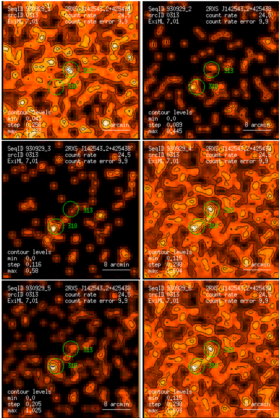
Figure 313: RASS 930929: detection 0313: band rate images, Gaussian filter: (1) PSPC channels 11 – 41, (2) 52 – 90, (3) 91 – 201, (4) 11 – 235, (5) 52 – 201, (6) 11 – 201. Broad band rates in counts/ks. Band rate contour levels in counts/ks/arcmin 2 .
