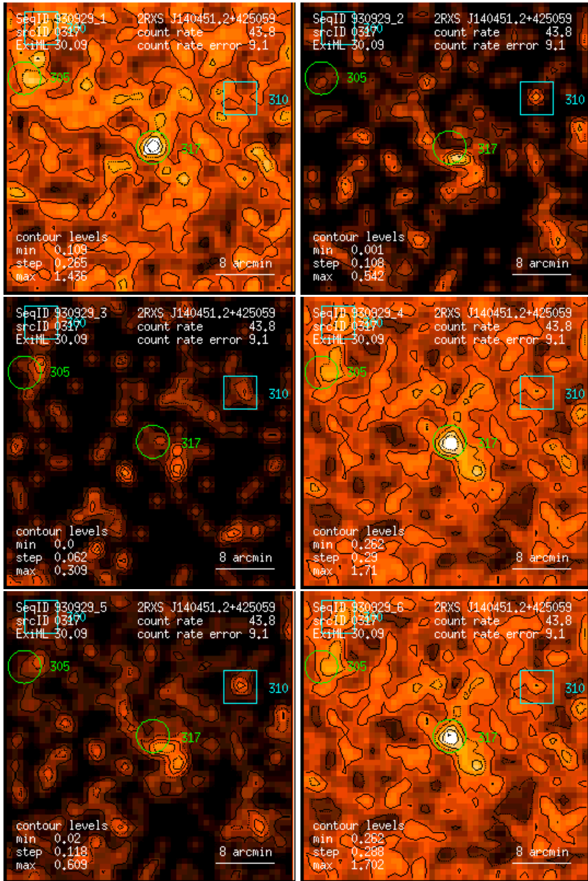
Figure 317: RASS 930929: detection 0317: band rate images, Gaussian filter: (1) PSPC channels 11 – 41, (2) 52 – 90, (3) 91 – 201, (4) 11 – 235, (5) 52 – 201, (6) 11 – 201. Broad band rates in counts/ks. Band rate contour levels in counts/ks/arcmin 2 .
