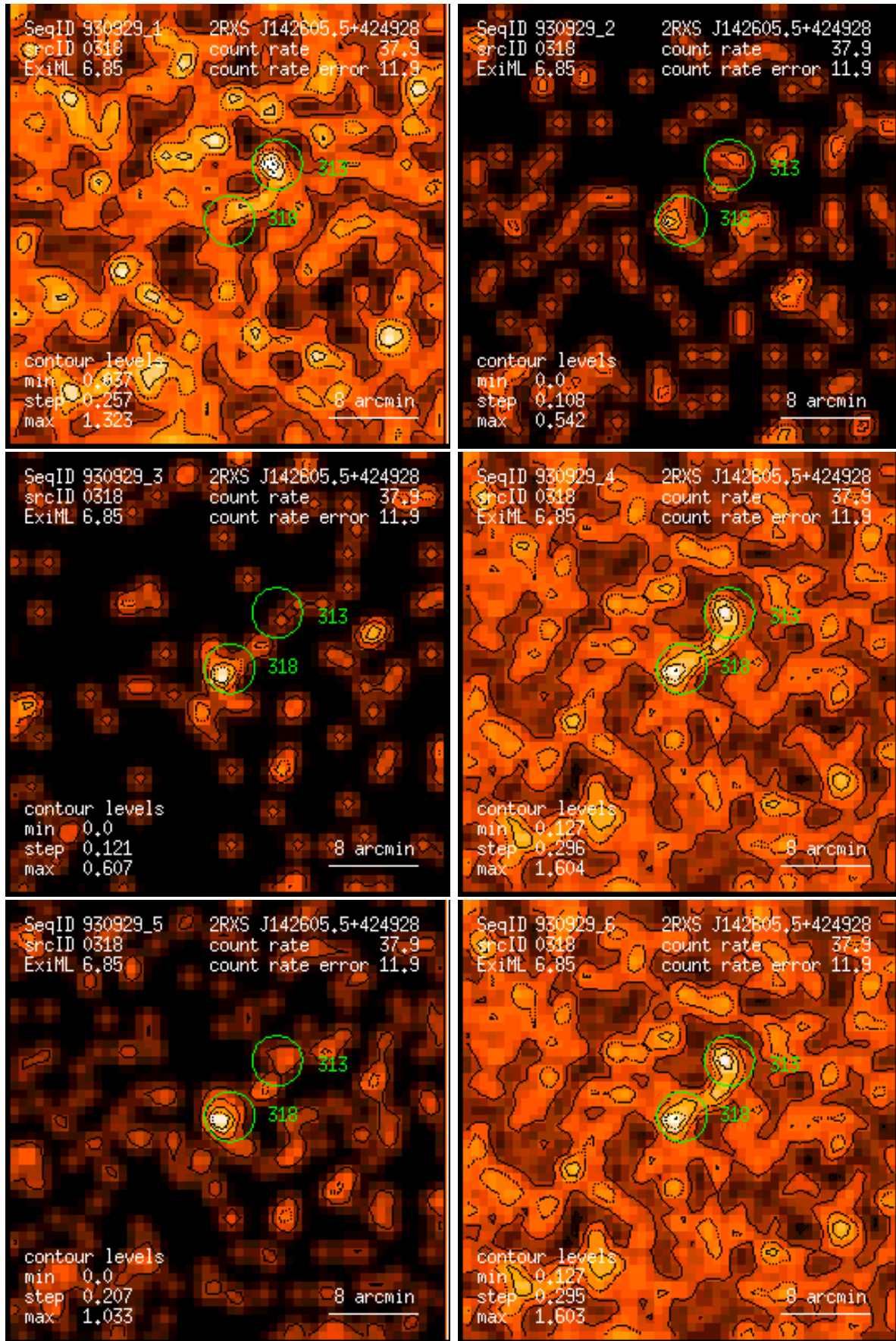
Figure 318: RASS 930929: detection 0318: band rate images, Gaussian filter: (1) PSPC channels 11 – 41, (2) 52 – 90, (3) 91 – 201, (4) 11 – 235, (5) 52 – 201, (6) 11 – 201. Broad band rates in counts/ks. Band rate contour levels in counts/ks/arcmin 2 .
