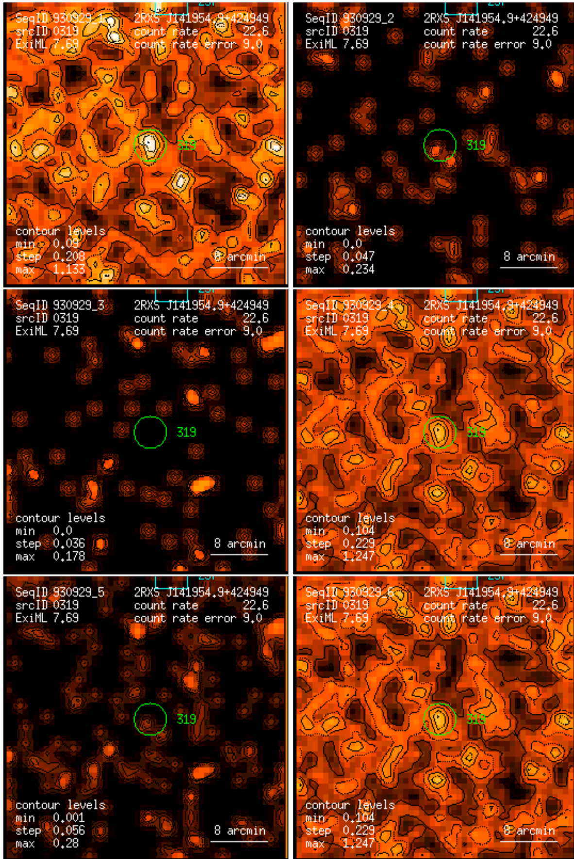
Figure 319: RASS 930929: detection 0319: band rate images, Gaussian filter: (1) PSPC channels 11 – 41, (2) 52 – 90, (3) 91 – 201, (4) 11 – 235, (5) 52 – 201, (6) 11 – 201. Broad band rates in counts/ks. Band rate contour levels in counts/ks/arcmin 2 .
