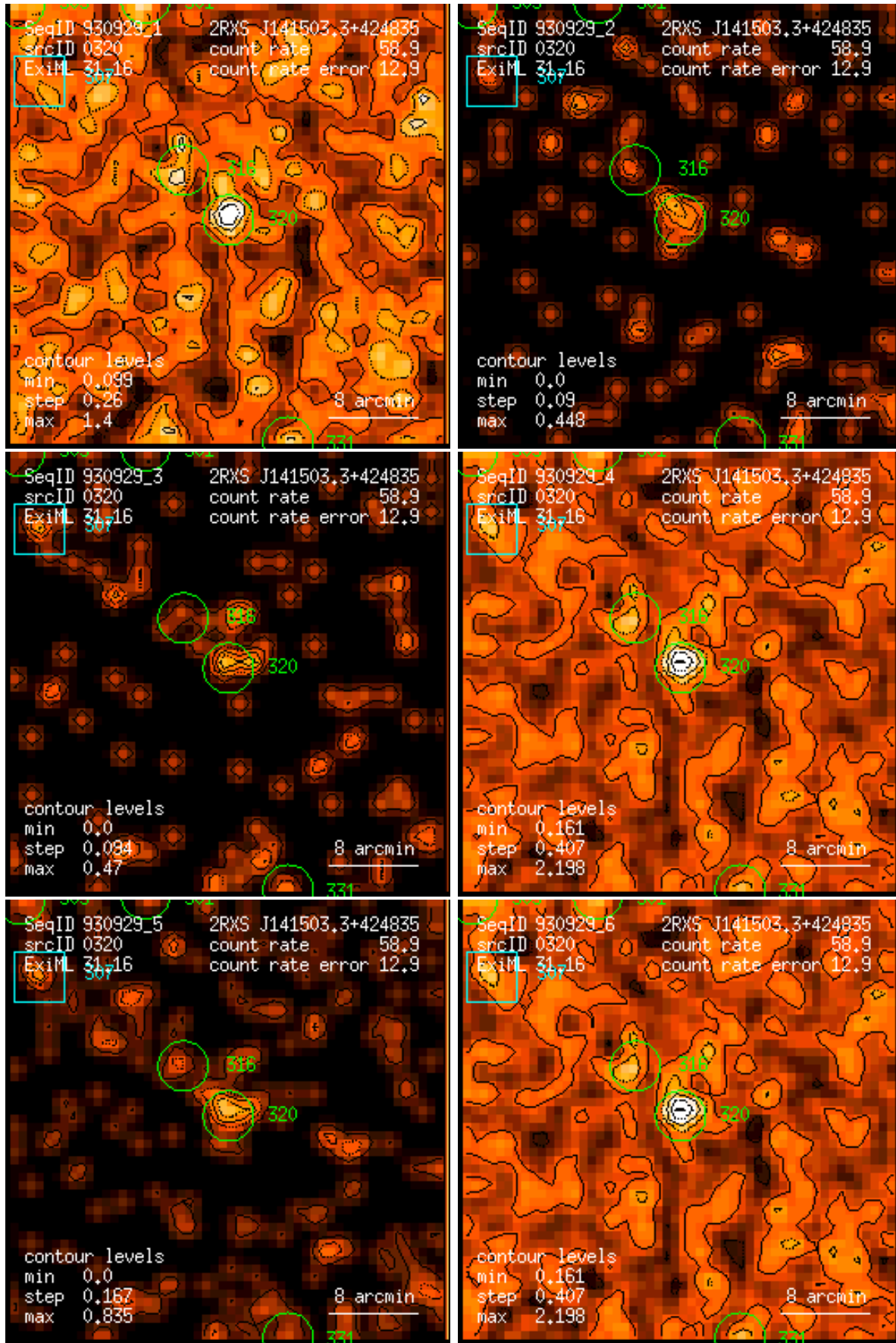
Figure 320: RASS 930929: detection 0320: band rate images, Gaussian filter: (1) PSPC channels 11 – 41, (2) 52 – 90, (3) 91 – 201, (4) 11 – 235, (5) 52 – 201, (6) 11 – 201. Broad band rates in counts/ks. Band rate contour levels in counts/ks/arcmin 2 .
