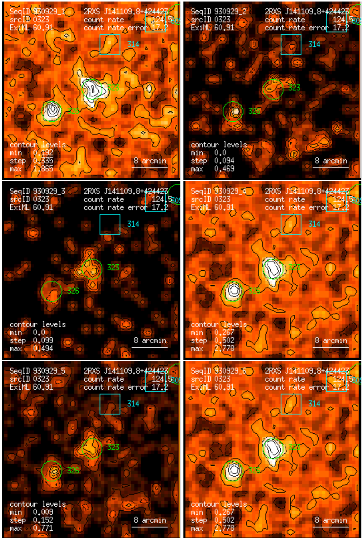
Figure 323: RASS 930929: detection 0323: band rate images, Gaussian filter: (1) PSPC channels 11 – 41, (2) 52 – 90, (3) 91 – 201, (4) 11 – 235, (5) 52 – 201, (6) 11 – 201. Broad band rates in counts/ks. Band rate contour levels in counts/ks/arcmin 2 .
