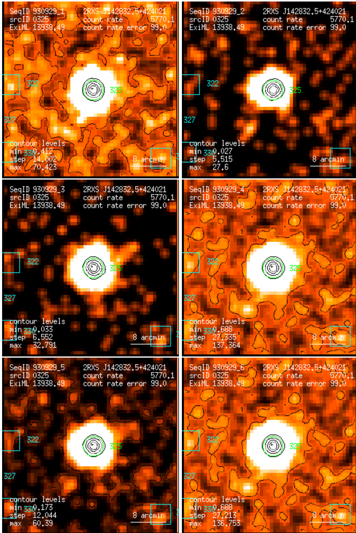
Figure 325: RASS 930929: detection 0325: band rate images, Gaussian filter: (1) PSPC channels 11 – 41, (2) 52 – 90, (3) 91 – 201, (4) 11 – 235, (5) 52 – 201, (6) 11 – 201. Broad band rates in counts/ks. Band rate contour levels in counts/ks/arcmin 2 .
