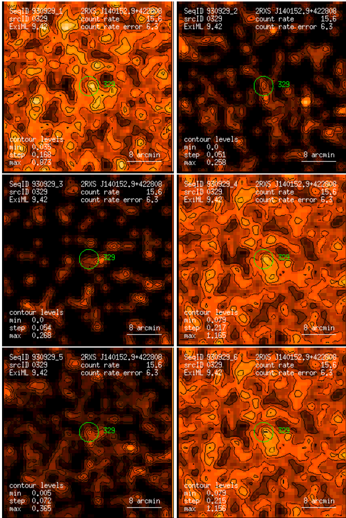
Figure 329: RASS 930929: detection 0329: band rate images, Gaussian filter: (1) PSPC channels 11 – 41, (2) 52 – 90, (3) 91 – 201, (4) 11 – 235, (5) 52 – 201, (6) 11 – 201. Broad band rates in counts/ks. Band rate contour levels in counts/ks/arcmin 2 .
