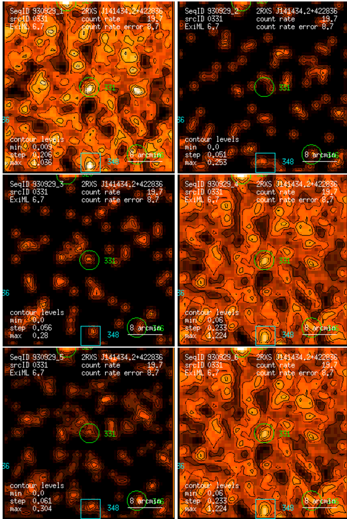
Figure 331: RASS 930929: detection 0331: band rate images, Gaussian filter: (1) PSPC channels 11 – 41, (2) 52 – 90, (3) 91 – 201, (4) 11 – 235, (5) 52 – 201, (6) 11 – 201. Broad band rates in counts/ks. Band rate contour levels in counts/ks/arcmin 2 .
