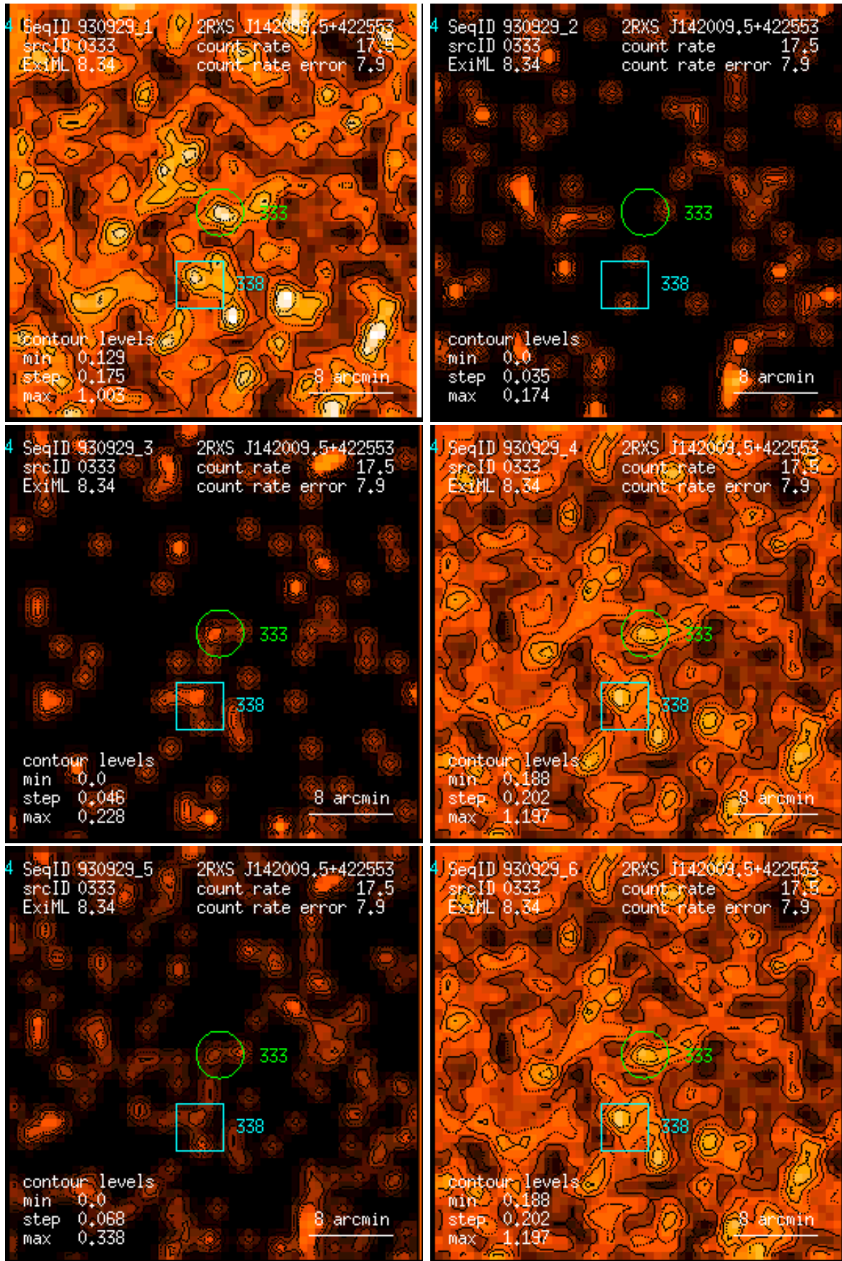
Figure 333: RASS 930929: detection 0333: band rate images, Gaussian filter: (1) PSPC channels 11 – 41, (2) 52 – 90, (3) 91 – 201, (4) 11 – 235, (5) 52 – 201, (6) 11 – 201. Broad band rates in counts/ks. Band rate contour levels in counts/ks/arcmin 2 .
