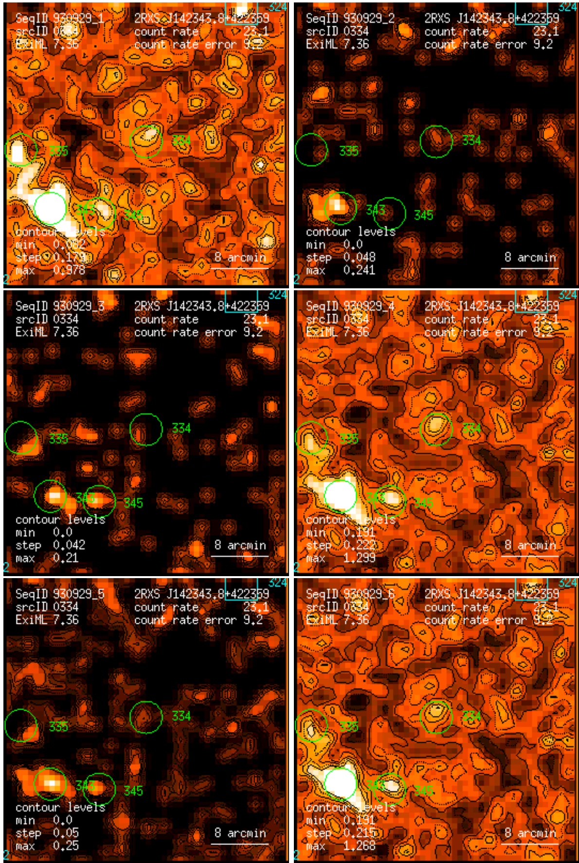
Figure 334: RASS 930929: detection 0334: band rate images, Gaussian filter: (1) PSPC channels 11 – 41, (2) 52 – 90, (3) 91 – 201, (4) 11 – 235, (5) 52 – 201, (6) 11 – 201. Broad band rates in counts/ks. Band rate contour levels in counts/ks/arcmin 2 .
