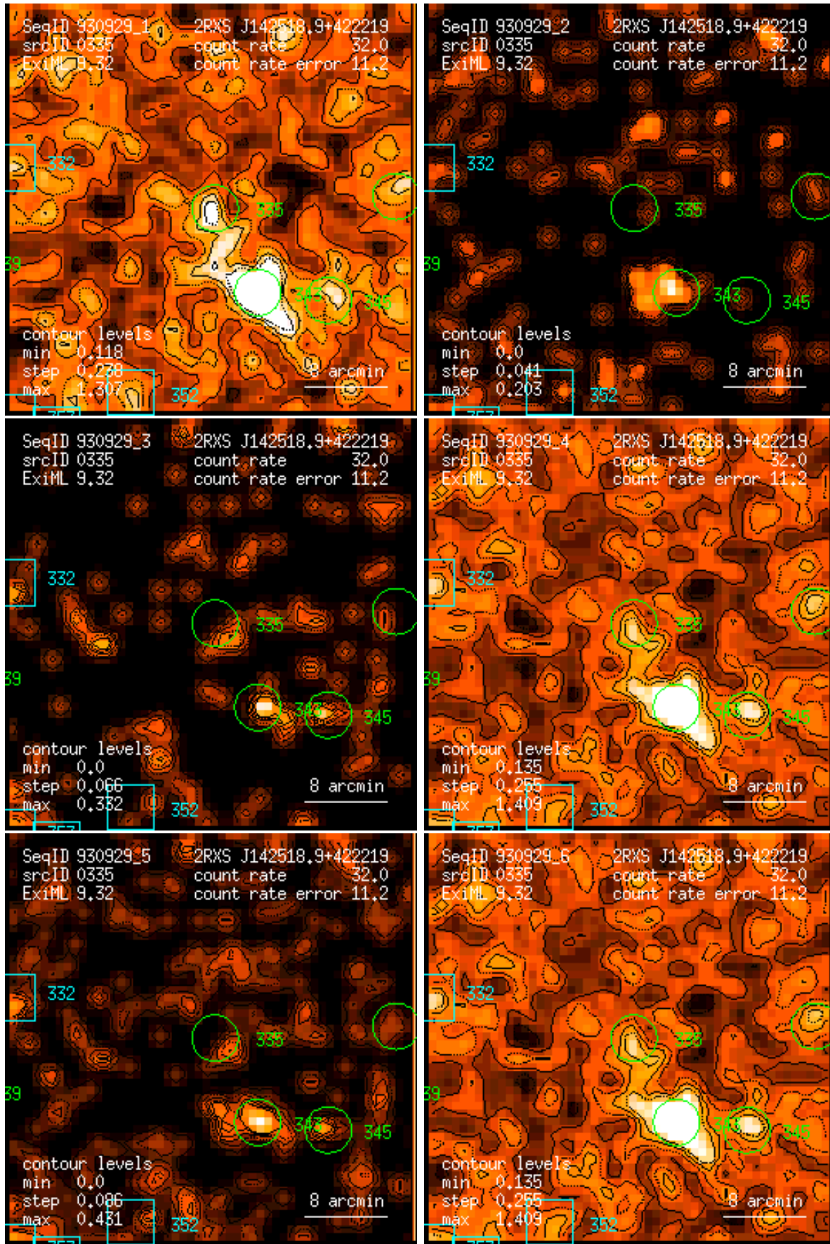
Figure 335: RASS 930929: detection 0335: band rate images, Gaussian filter: (1) PSPC channels 11 – 41, (2) 52 – 90, (3) 91 – 201, (4) 11 – 235, (5) 52 – 201, (6) 11 – 201. Broad band rates in counts/ks. Band rate contour levels in counts/ks/arcmin 2 .
