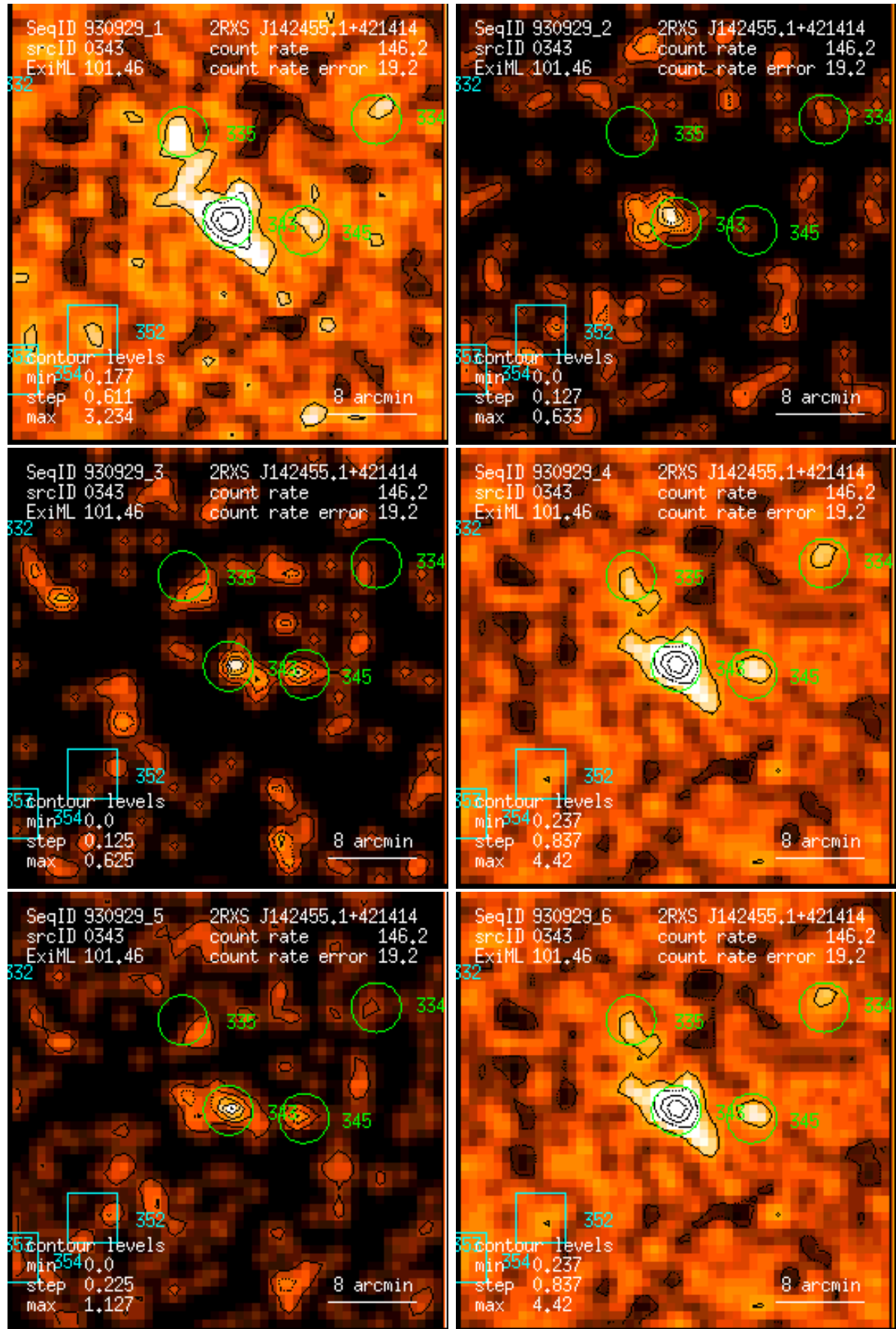
Figure 343: RASS 930929: detection 0343: band rate images, Gaussian filter: (1) PSPC channels 11 – 41, (2) 52 – 90, (3) 91 – 201, (4) 11 – 235, (5) 52 – 201, (6) 11 – 201. Broad band rates in counts/ks. Band rate contour levels in counts/ks/arcmin 2 .
