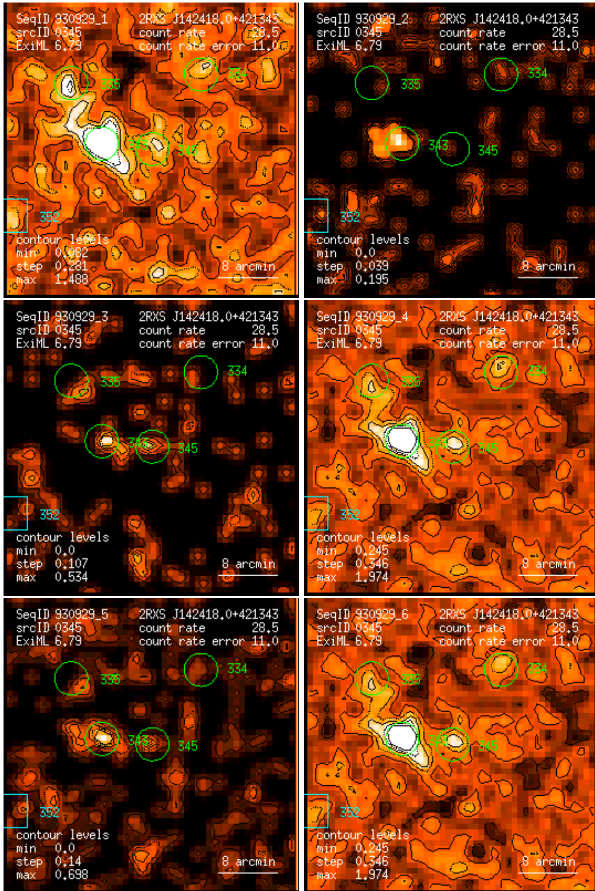
Figure 345: RASS 930929: detection 0345: band rate images, Gaussian filter: (1) PSPC channels 11 – 41, (2) 52 – 90, (3) 91 – 201, (4) 11 – 235, (5) 52 – 201, (6) 11 – 201. Broad band rates in counts/ks. Band rate contour levels in counts/ks/arcmin 2 .
