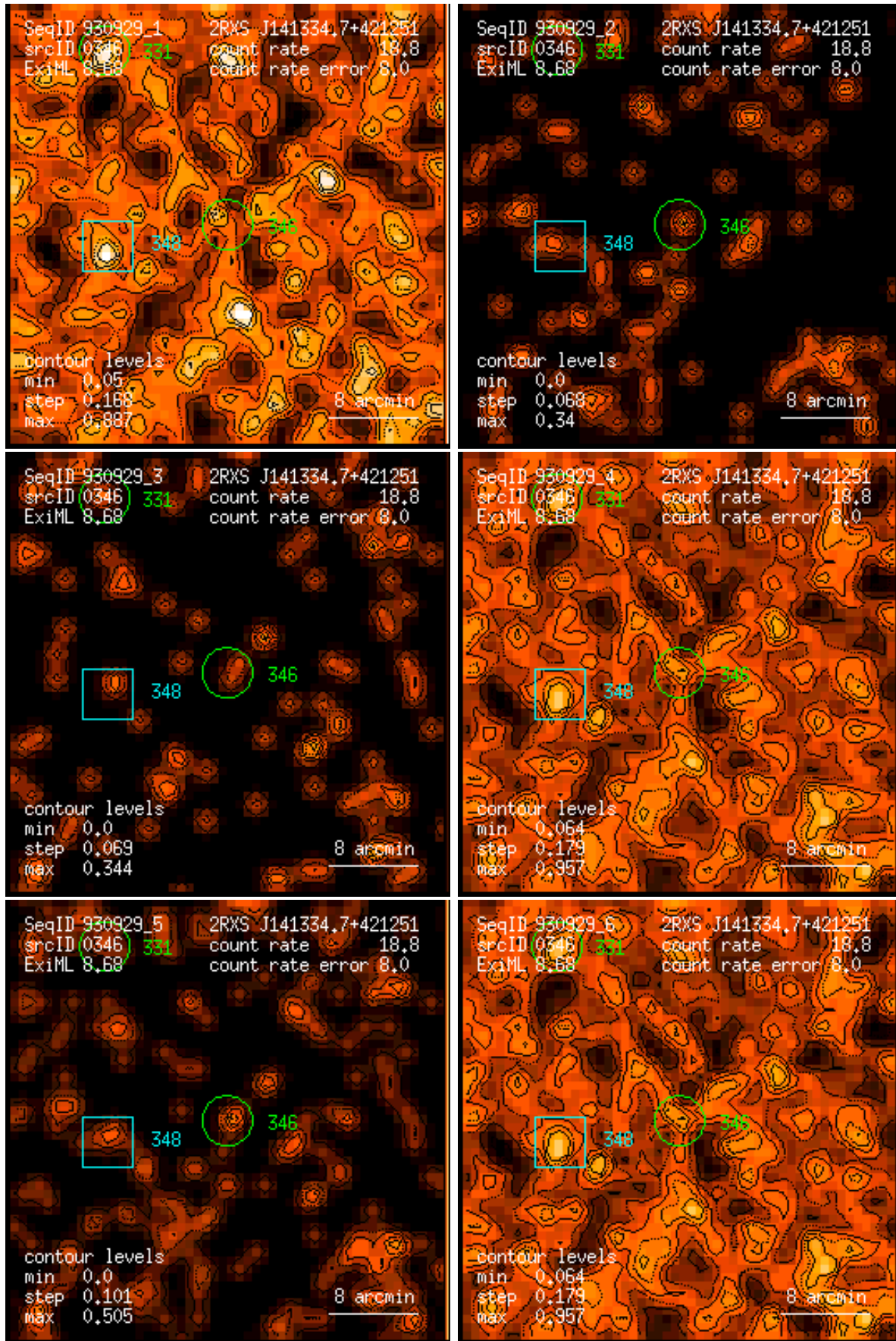
Figure 346: RASS 930929: detection 0346: band rate images, Gaussian filter: (1) PSPC channels 11 – 41, (2) 52 – 90, (3) 91 – 201, (4) 11 – 235, (5) 52 – 201, (6) 11 – 201. Broad band rates in counts/ks. Band rate contour levels in counts/ks/arcmin 2 .
