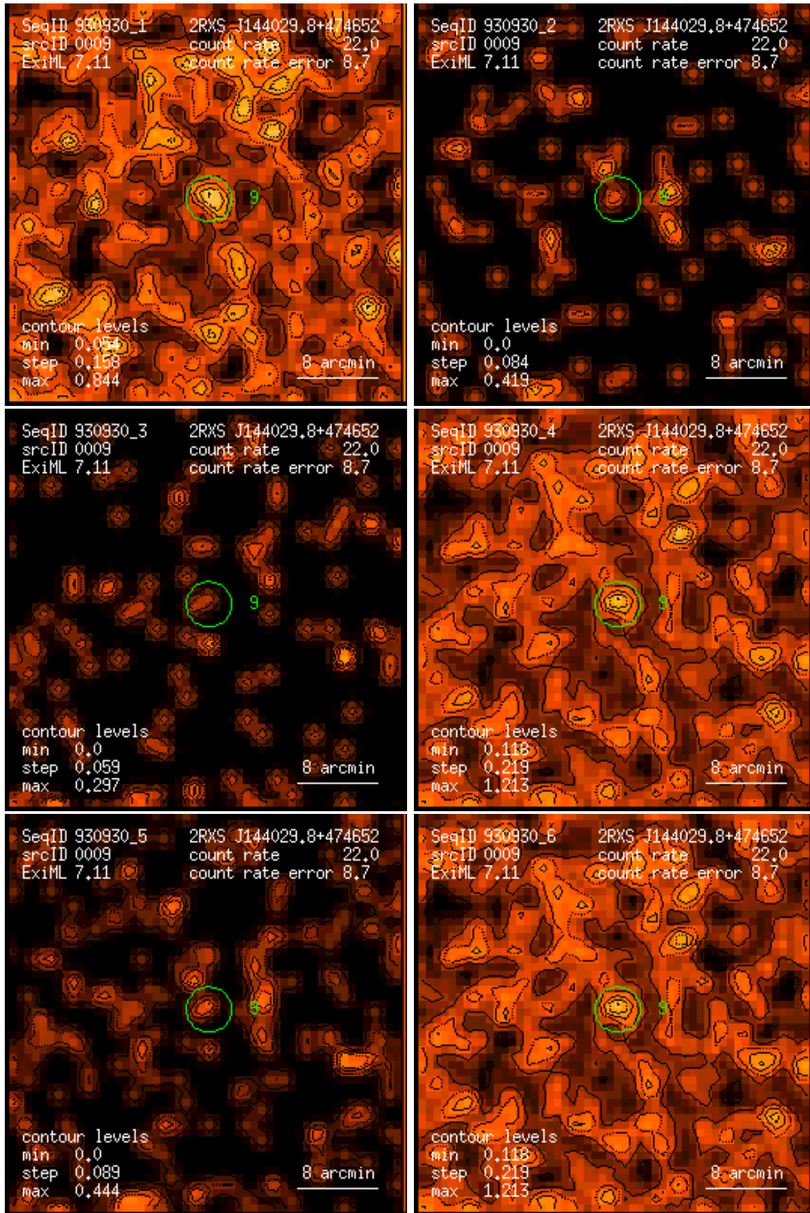
Figure 9: RASS 930930: detection 0009: band rate images, Gaussian filter: (1) PSPC channels 11 – 41, (2) 52 – 90, (3) 91 – 201, (4) 11 – 235, (5) 52 – 201, (6) 11 – 201. Broad band rates in counts/ks. Band rate contour levels in counts/ks/arcmin 2 .
