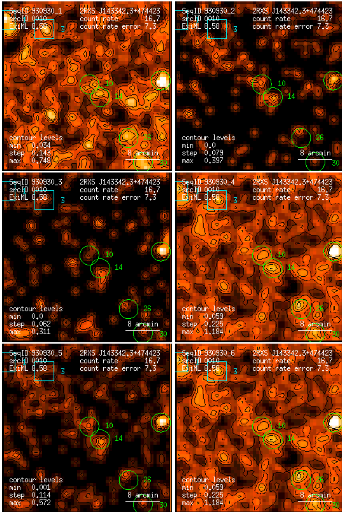
Figure 10: RASS 930930: detection 0010: band rate images, Gaussian filter: (1) PSPC channels 11 – 41, (2) 52 – 90, (3) 91 – 201, (4) 11 – 235, (5) 52 – 201, (6) 11 – 201. Broad band rates in counts/ks. Band rate contour levels in counts/ks/arcmin 2 .
