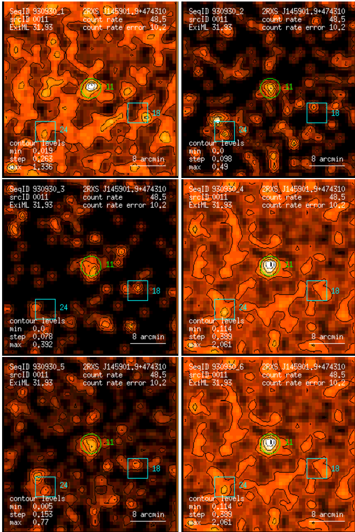
Figure 11: RASS 930930: detection 0011: band rate images, Gaussian filter: (1) PSPC channels 11 – 41, (2) 52 – 90, (3) 91 – 201, (4) 11 – 235, (5) 52 – 201, (6) 11 – 201. Broad band rates in counts/ks. Band rate contour levels in counts/ks/arcmin 2 .
