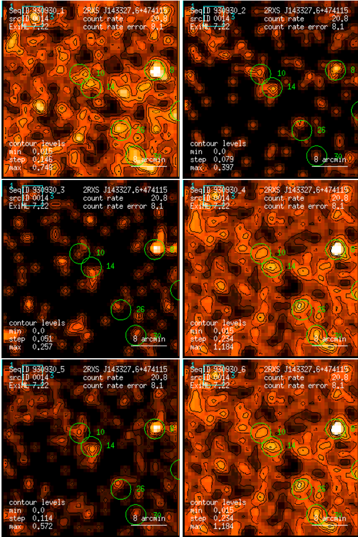
Figure 14: RASS 930930: detection 0014: band rate images, Gaussian filter: (1) PSPC channels 11 – 41, (2) 52 – 90, (3) 91 – 201, (4) 11 – 235, (5) 52 – 201, (6) 11 – 201. Broad band rates in counts/ks. Band rate contour levels in counts/ks/arcmin 2 .
