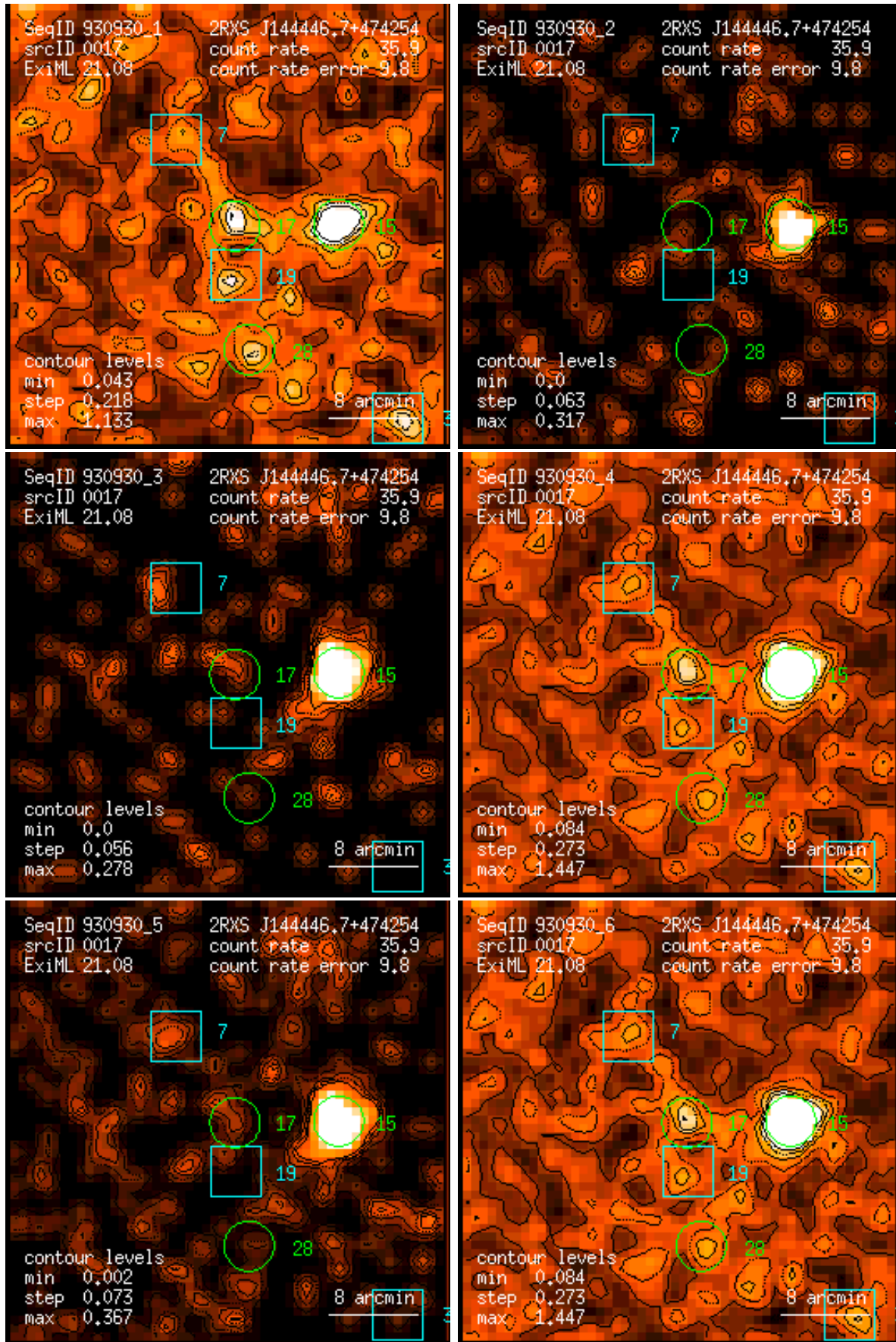
Figure 17: RASS 930930: detection 0017: band rate images, Gaussian filter: (1) PSPC channels 11 – 41, (2) 52 – 90, (3) 91 – 201, (4) 11 – 235, (5) 52 – 201, (6) 11 – 201. Broad band rates in counts/ks. Band rate contour levels in counts/ks/arcmin 2 .
