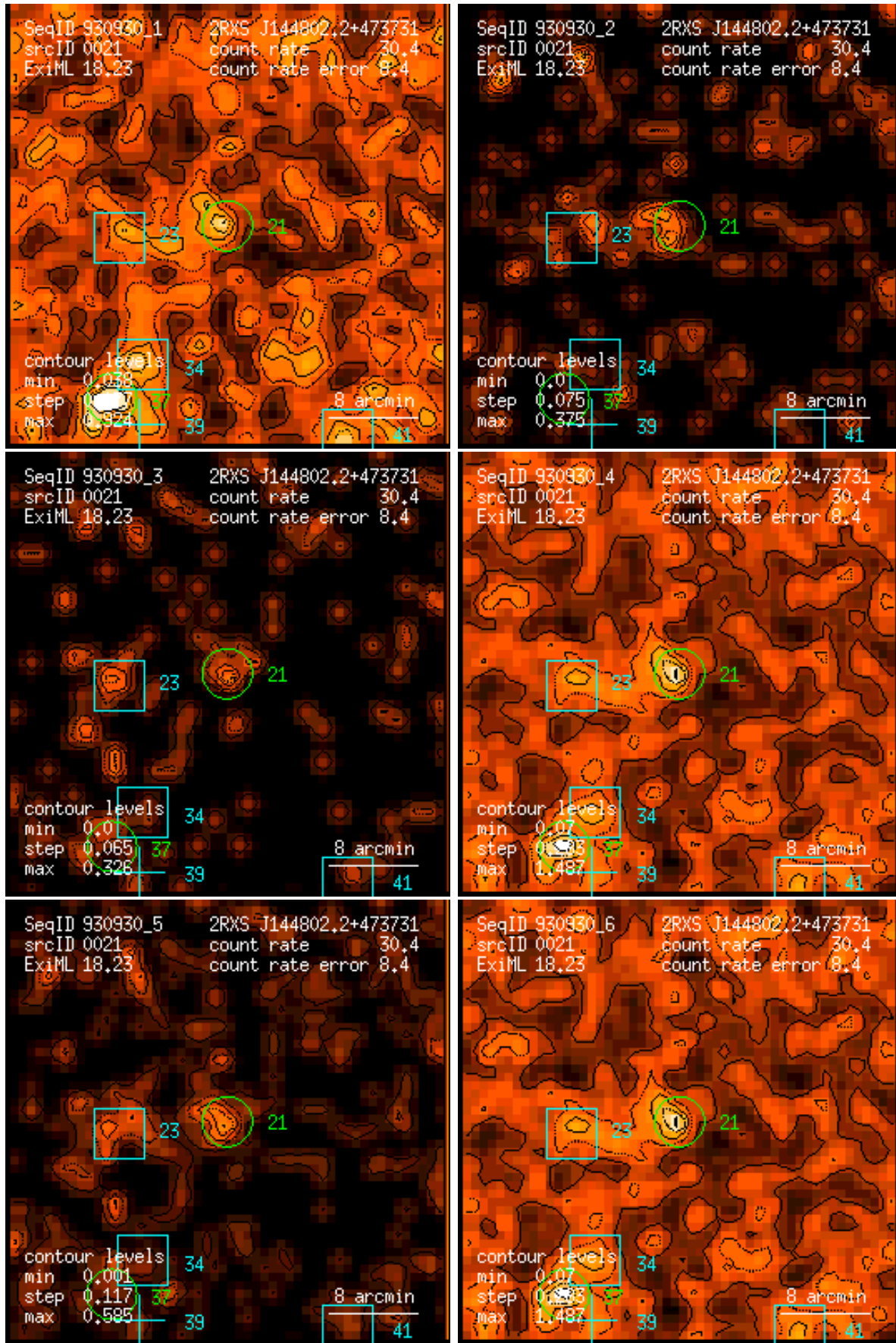
Figure 21: RASS 930930: detection 0021: band rate images, Gaussian filter: (1) PSPC channels 11 – 41, (2) 52 – 90, (3) 91 – 201, (4) 11 – 235, (5) 52 – 201, (6) 11 – 201. Broad band rates in counts/ks. Band rate contour levels in counts/ks/arcmin 2 .
