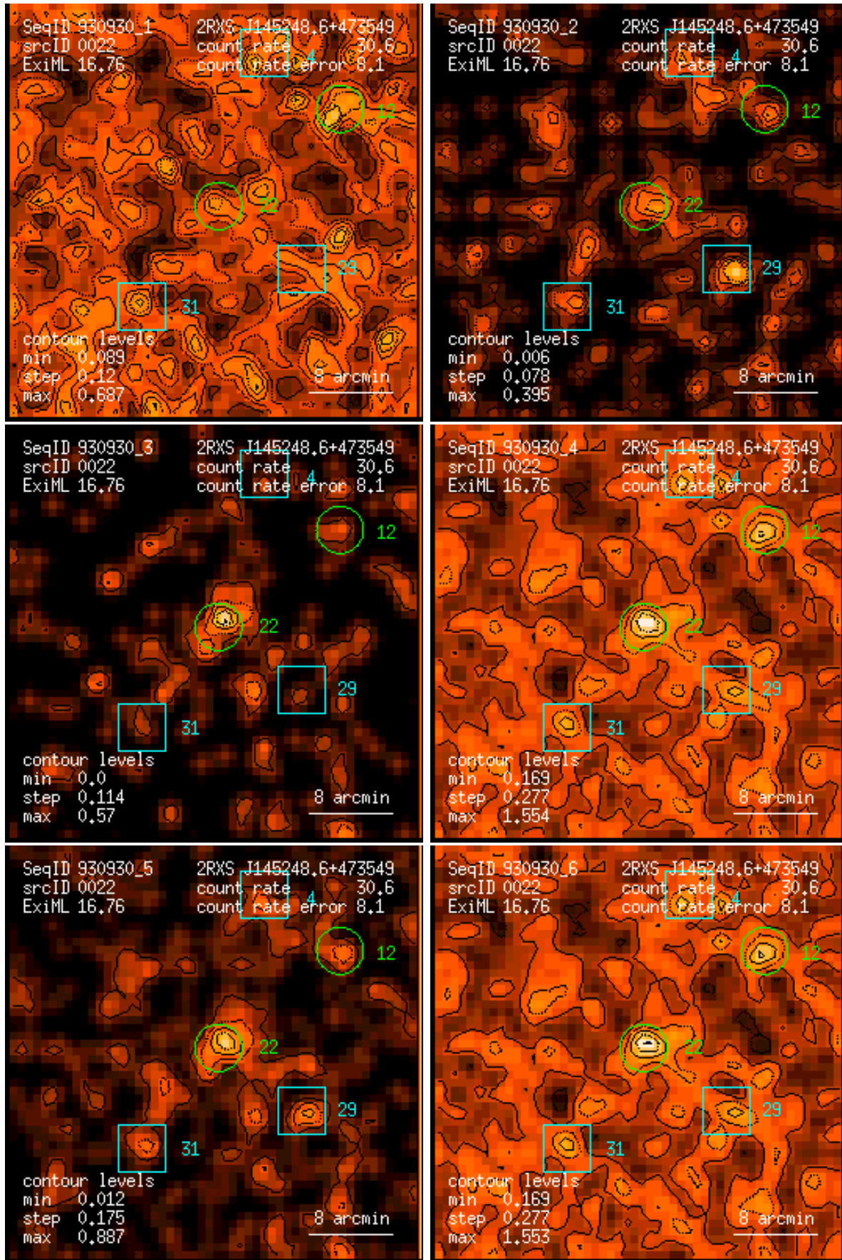
Figure 22: RASS 930930: detection 0022: band rate images, Gaussian filter: (1) PSPC channels 11 – 41, (2) 52 – 90, (3) 91 – 201, (4) 11 – 235, (5) 52 – 201, (6) 11 – 201. Broad band rates in counts/ks. Band rate contour levels in counts/ks/arcmin 2 .
